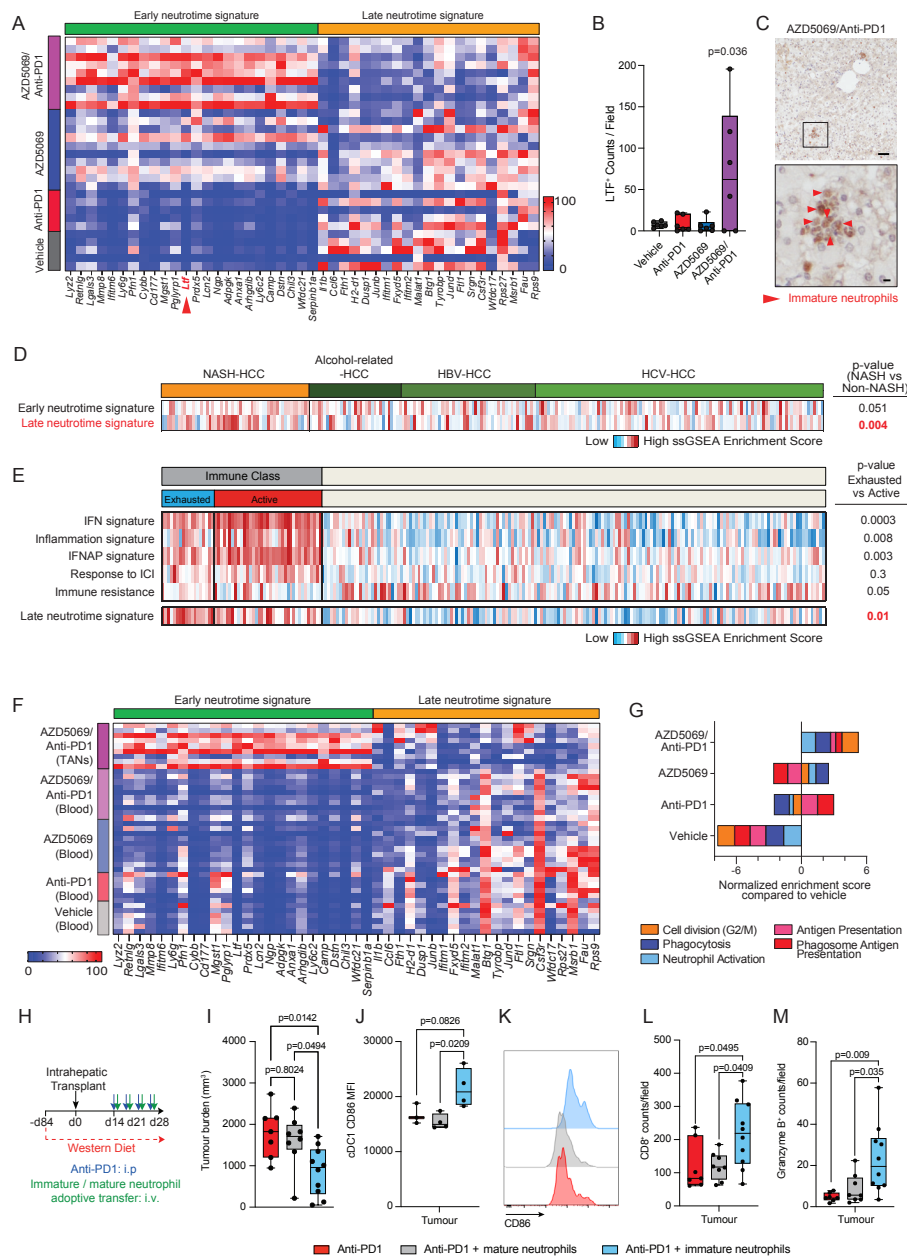
Figure 6 AZD5069/anti-PD1 combination therapy reprogrammes the TAN phenotype. (A) Heatmap showing row-scaled expression of genes associated with late and early neutrotime for DEN/ALIOS mice TANs. (B) Quantification of LTF + counts/field by IHC for DEN/ALIOS mice tumours at day 284. (C) Representative image of LTF positive neutrophils (red arrow) in the tumour of AZD5069/anti-PD1 treated DEN/ALIOS mice at day 284. Scale bar top = 100 \mu m, bottom = 10 \mu m. (D) Heatmap showing row-scaled expression of early and late neutrotime signatures for human NASH-HCC compared with HBV, HCV and alcohol-related HCC (non-NASH-HCC). In total n=237 patients analysed. (E) Heatmap showing row-scaled expression of published HCC immune class signatures; IFN, inflammation, IFNAP, Response to ICI and immune resistance as well as the late neutrotime signature for human HCC active and exhausted immune subsets. In total n=228 patients analysed. (F) Heatmap showing row-scaled expression of genes associated with late and early neutrotime signatures for DEN/ALIOS peripheral blood neutrophils and AZD5069/Anti-PD1 treated TANs. (G) Gene set enrichment analysis (GSEA) showing normalised enrichment scores for TAN process networks highly enriched in; Anti-PD1 vs Vehicle (Phagosome Antigen Presentation and Antigen Presentation), AZD5069 vs Vehicle (Neutrophil Activation and Phagocytosis), and AZD5069/Anti-PD1 vs Vehicle (G2-M). (H) Timeline schematic for neutrophil based therapy treatment regime in the orthotopic NASH-HCC model. (I) Quantification of tumour burden in orthotopic NASH-HCC mice treated with anti-PD1 and immature or mature neutrophils at day 28 post-intrahepatic injection. (J, K) Flow cytometric quantification and representative histogram plot of CD86 median fluorescent intensity (MFI) of intratumoural XCR1 + cDC1 cells from orthotopic NASH-HCC neutrophil/anti-PD1 therapy mice at day 28. (L, M) Quantification of intratumoural CD8 + and granzyme B + counts/field in the tumours of orthotopic NASH-HCC neutrophil/anti-PD1 therapy mice at day 28. Data are from: Bulk DEN/ALIOS Ly6G + TAN RNA-Seq data in (A, F, G) and bulk tumour microarray in (D, E). Dots in (B, I, J, L, M) represent individual mice. Significance tested using: One-Way ANOVA with Tukey’s multiple comparisons test (B, I, J, L, M). Exact p-values indicated on graph. ALIOS, American lifestyle induced obesity syndrome diet; ANOVA, analysis of variance; DEN, Diethylnitrosamine; HCC, hepatocellular carcinoma; IHC, immunohistochemistry; ICI, immune checkpoint inhibition; NASH, non-alcoholic steatohepatitis; TANs, tumour-associated neutrophils.
