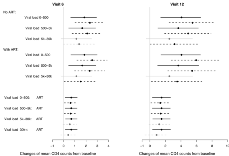
FIGURE 2 Results (posterior means and 95% credible intervals) for marginal covariate effects on changes of mean square root CD4 counts from baseline to visits 6 and 12 in the HERS analysis. Top: baseline viral load effects on mean CD4 count changes, given baseline ART status. Bottom: baseline ART status effects on mean CD4 count changes, given baseline viral load levels. Solid lines (—): 95% credible intervals under the default extrapolation distribution of the SPM; dashed lines (----): 95% credible intervals under the extrapolation distribution in the sensitivity analysis. The estimated effects with 95% credible intervals covering zero and not covering zero are in gray and black, respectively.
