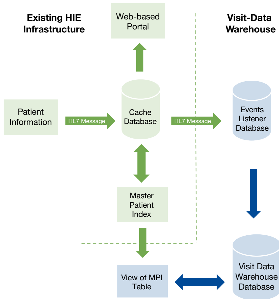
Figure 1. Workflow Diagram for the Interaction between the VDW and the Primary HIE Infrastructure
