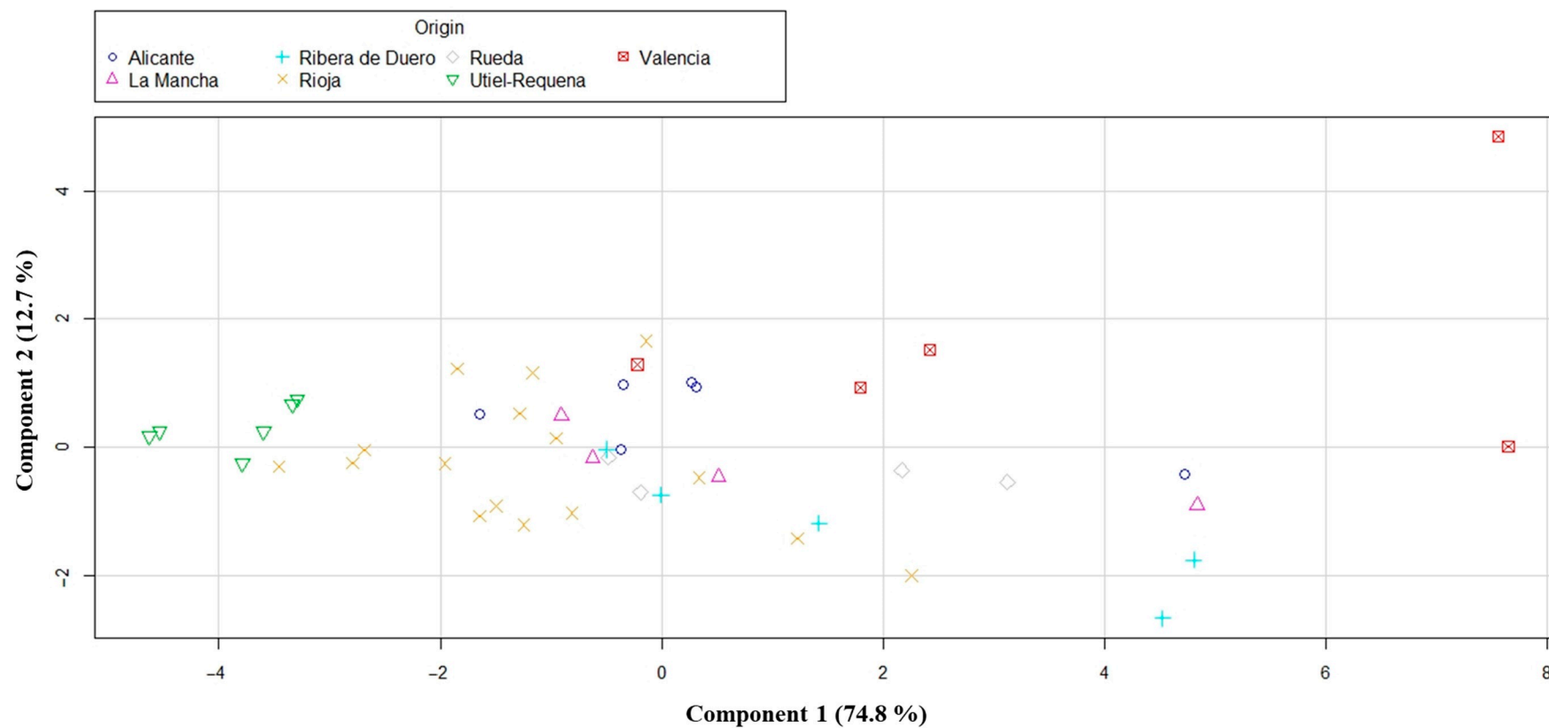
Figure 1. Principal components analysis performed on data expressed as concentration of REEs (Dy, Er, Eu, Gd, Ho, Nd, Pr, Sm, Tb, Tm and Yb) in wines from different designations of origin. (a) Loading plot; (b) score plot.
