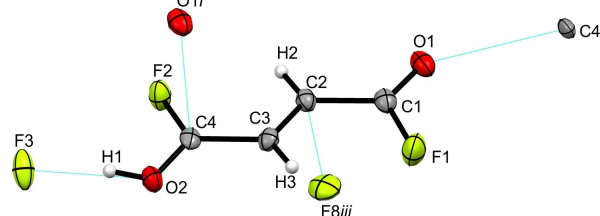
Figure 3. Illustration of the cation in [\text{C}_4\text{H}_3\text{F}_2\text{O}_2]^+[\text{SbF}_6]^- and its interatomic contacts (displacement ellipsoids with 50% probability). Symmetry operations: i = 0.5 + x, 1.5 - y, -0.5 + z ; ii = -0.5 + x, 1.5 - y, 0.5 + z ; iii = -1 + x, 1 - y, 0.5 + z . Interatomic contacts are shown as dashed blue lines.
