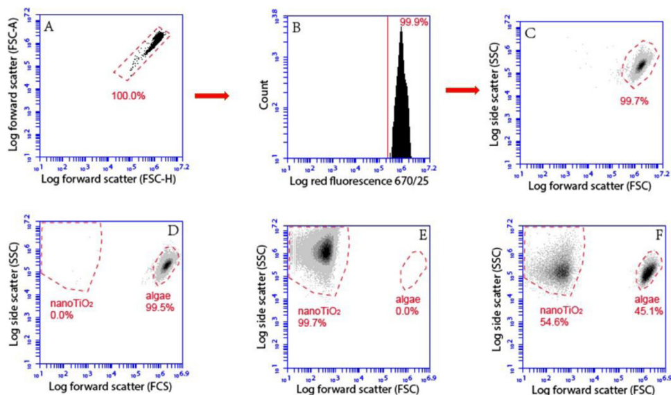
Fig. 4. Schematic representation of the FCM data analysis procedure used to define the gate corresponding to algae and nanoTiO 2 aggregates. As a first step FSC-H/FSC-A dot-plot (A) was used to remove eventual instrument background. Then signals present in the gated region were plotted in a count versus red fluorescence plot (B) and SSC/FSC dot-plot (C) to verify cellular characteristics of size, granularity and chlorophyll autofluorescence. (D) cytogram of algal suspension ( 1.0 \times 10^6 cells/mL) in the absence of nanoTiO 2 , (E) cytogram of 200 mg L -1 nanoTiO 2 suspension only (F) cytogram of mixture containing 1.0 \times 10^6 cells/mL algae and 200 mg L -1 nanoTiO 2 .
