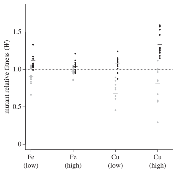
Figure 2. The relative fitness of mutants compared with wild-type ( W ) depends on an interaction between metal species (copper or iron) and growth conditions (monoculture, grey; co-culture, black; two-way interaction between metal and growth conditions: F_{1,88} = 30.583 , p < 0.001 ), and an interaction between metal species and metal concentration (high = 6.17 mM, low = 624 \mu\text{M} ; two-way interaction between metal species and concentration, F_{1,88} = 11.612 , p < 0.001 ). In co-culture, W > 1 (i.e. mutants invade) for highly toxic copper concentrations (one-sample t -test on relative fitness, alternative = 1, t_{11} = 7.3307 , p < 0.001 ).
