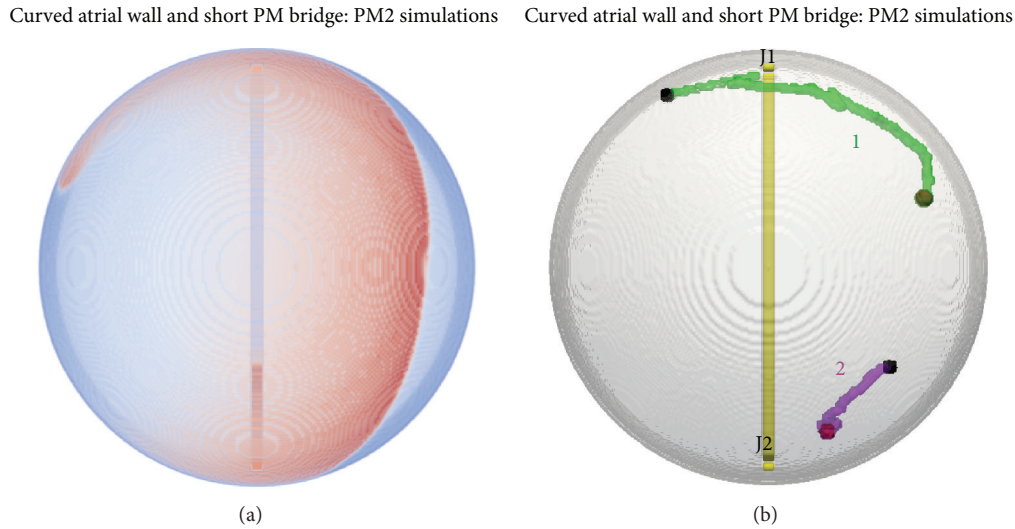
FIGURE 9: Curved wall bridge simulations. (a) Representative snapshot. The reentry looks distorted as it is on the steep part of the hemispherical wall, at a large angle to the presented view. (b) Two tip traces from simulations where scroll waves were initiated on either side of the bridge junctions. J1 and J2 indicate junctions of the PM bridge with the atrial wall on the endocardial side of the model.
