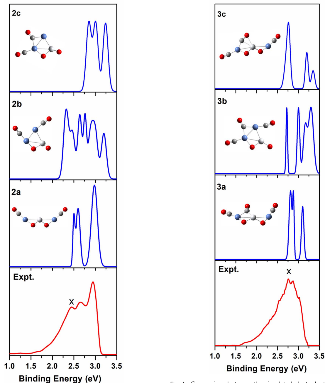
Fig. 4 Comparison between the simulated photoelectron spectra of the three \text{Ni}_2\text{TiO}_2(\text{CO})_3^- isomers 3a , 3b , 3c (blue line) and the experimental one at 355 nm (red line).
