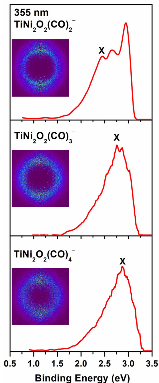
Fig. 1 Photoelectron images of \text{Ni}_2\text{TiO}_2(\text{CO})_n^- ( n = 2-4 ) at 355 nm. Photoelectron images after inverse Abel transformation are embedded in the photoelectron spectra.
