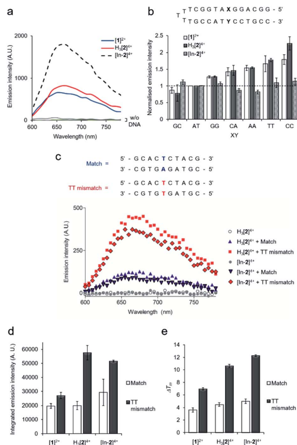
Fig. 2 (a) MLCT luminescence of Ru(II) complexes (30 \mu\text{M} ) without (w/o) and with calf-thymus DNA (80 \mu\text{M} ) ( \lambda_{\text{ex}} = 405 \text{ nm} ). (b) Relative emission intensities for [\text{1}]^{2+} , \text{H}_3[\text{2}]^{4+} or [\text{In-2}]^{4+} (30 \mu\text{M} ) with the addition of DNA hairpins containing a single variable XY base pair (3 \mu\text{M} , top). Data for each compound normalised to XY = AT emission intensity (dashed line). Mean of two independent replicates \pm S.D. (c) Emission spectra of \text{H}_3[\text{2}]^{4+} or [\text{In-2}]^{4+} with 10-mer matched DNA duplex or 10-mer containing a single TT mismatch site (duplex sequences shown at top, 30 \mu\text{M} complex, 3 \mu\text{M} DNA duplex). (d) Integrated emission intensities TT mismatch and matched DNA with the addition of [\text{1}]^{2+} , \text{H}_3[\text{2}]^{4+} or [\text{In-2}]^{4+} (3 \mu\text{M} DNA duplexes, 30 \mu\text{M} complexes). Average of two independent experiments \pm S.D. (e) \Delta T_m ( ^\circ\text{C} ) values for match or TT mismatch duplexes (3 \mu\text{M} ) with the addition of complexes (30 \mu\text{M} ), determined by thermal denaturation studies (each T_m average of six successive melting curves per condition). T_m (match) = 47.43^\circ\text{C} , T_m (TT mismatch) = 33.62^\circ\text{C} . Error bars represent the combined standard uncertainty. Conditions: 10 mM phosphate buffer, 200 mM NaCl, pH 7.0. \lambda_{\text{ex}} = 405 \text{ nm} , \lambda_{\text{em}} = 600\text{--}800 \text{ nm} for [\text{1}]^{2+} , \text{H}_3[\text{2}]^{4+} and [\text{In-2}]^{4+} .
