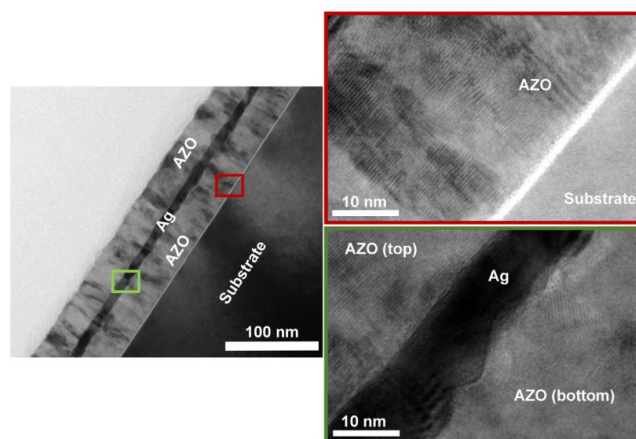
Figure 1. The cross-sectional TEM image of AZO/Ag/AZO [18].
