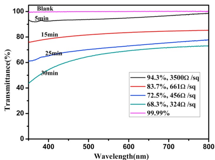
Figure 10. UV-VIS spectra of graphene films grown on glass with varying growth time (5, 15, 25, and 30 min) and the corresponding sheet resistance [50].
