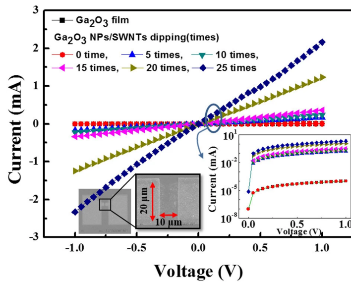
Figure 6. Current–voltage characteristic curves [41].
