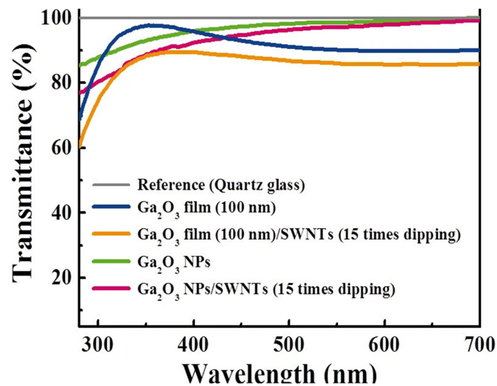
Figure 7. Optical transmittance spectra of undoped Ga 2 O 3 film [41].
