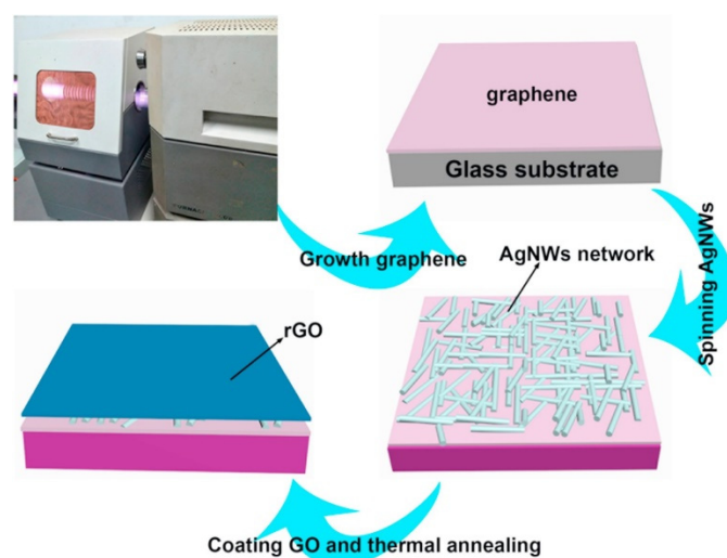
Figure 9. Schematic of the fabrication process of the G/Ag NWs/G sandwich film on a glass substrate [50].
