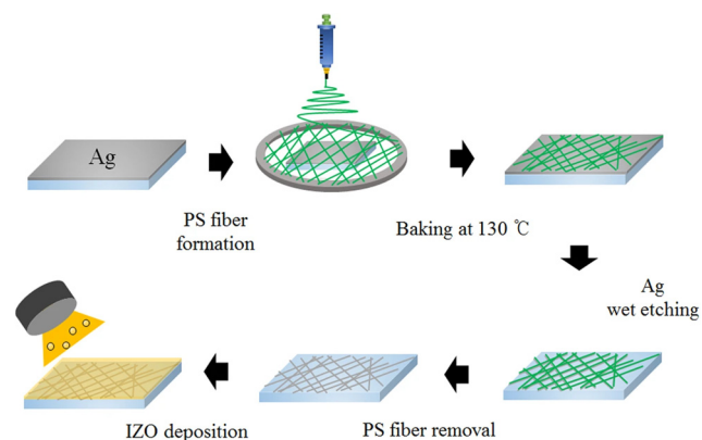
Figure 3. Schematic illustration of the fabrication procedure of Ag fiber/IZO composite electrodes [35].
