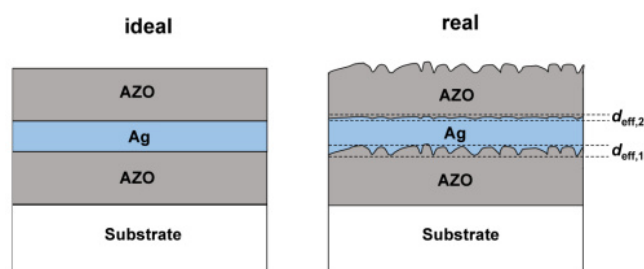
Figure 2. The ideal interfaces and real interfaces [18].
