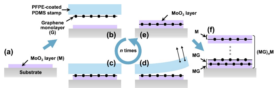
Figure 8. Schematic of the fabrication of \text{MoO}_3 -interlayer-doped graphene multilayers [47]. Thermally deposited a \text{MoO}_3 layer on a substrate (a). A graphene monolayer deposited on a PFPE-coated PDMS stamp by a modified wet-transfer method is transferred onto the \text{MoO}_3 layer by a transfer-printing process [(b–d)]. Next, another \text{MoO}_3 layer is deposited on the transfer-printed graphene layer (e). By performing steps (b) through (e) n times, (\text{MG})_n\text{M} is obtained (f).
