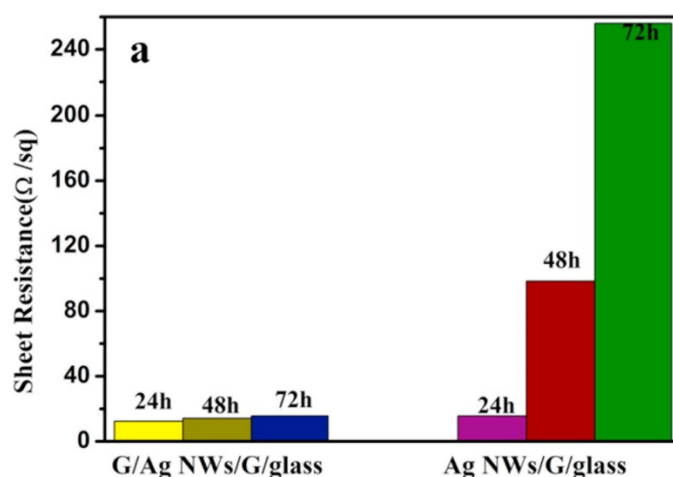
Figure 11. Changes of sheet resistance of G/AgNWs/G/glass and AgNWs/G/glass after exposure to air at 95 °C for 24, 48, and 72 h [50]. The original figure is from reference [50], figure 11 (a).
