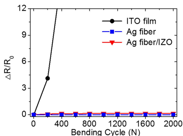
Figure 4. Resistance changes in the cyclic bending test [35].
