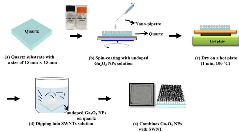
Figure 5. The schematic illustration for spin and dip-coating procedure of proposed Ga 2 O 3 -NP/SWNT layer on quartzes [41].
