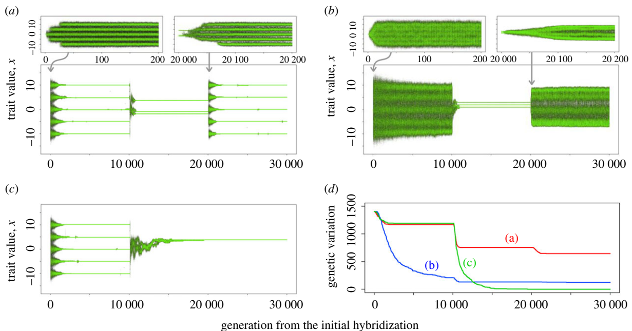
Figure 4. Simulation examples with the temporally repeated AR scenario. (a) With strong divergent selection in AR ( \varphi_B = 0.2 ) and complete isolation of refugia ( m_R = 0 ). (b) With weak divergent selection in AR ( \varphi_B = 0.0125 ) and complete isolation of refugia ( m_R = 0 ). (c) With strong divergent selection in AR ( \varphi_B = 0.2 ) and incomplete isolation of refugia ( m_R = 0.001 ). (d) Numbers of remaining SNPs at each generation in the three simulation examples. Other parameters: default values in electronic supplementary material, table S1.
