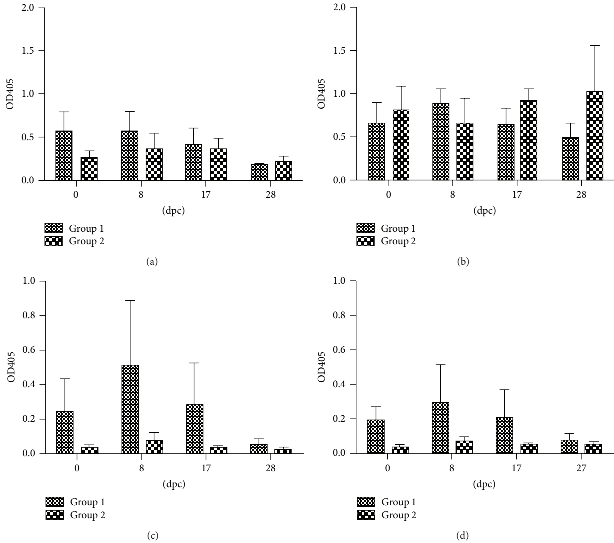
FIGURE 2: IgG ((a), (b)) and IgA ((c), (d)) antibodies against \gamma -intimin C280 ((a), (c)) and EspB ((b), (d)) in calves challenged with 10 8 or 10 10 CFU of E. coli O157:H7. Data are shown as mean OD405 \pm S.E.M.
