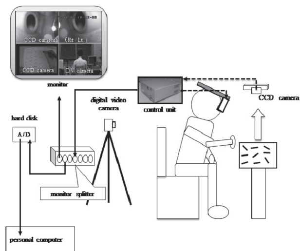
Fig. 2. Experimental apparatus
