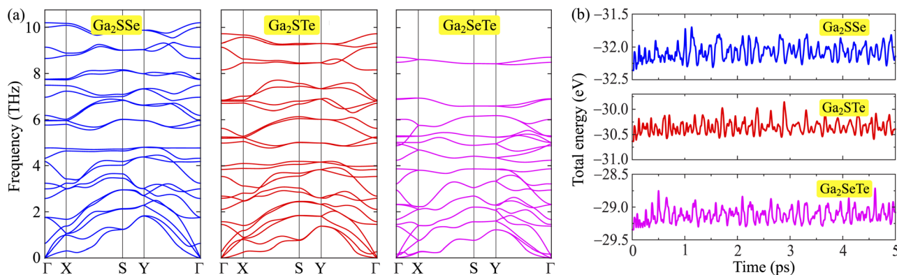
Fig. 2 (a) Phonon spectra and (b) AIMD calculation for the variations of the total energy to time of Janus Ga 2 XY at room temperature.
