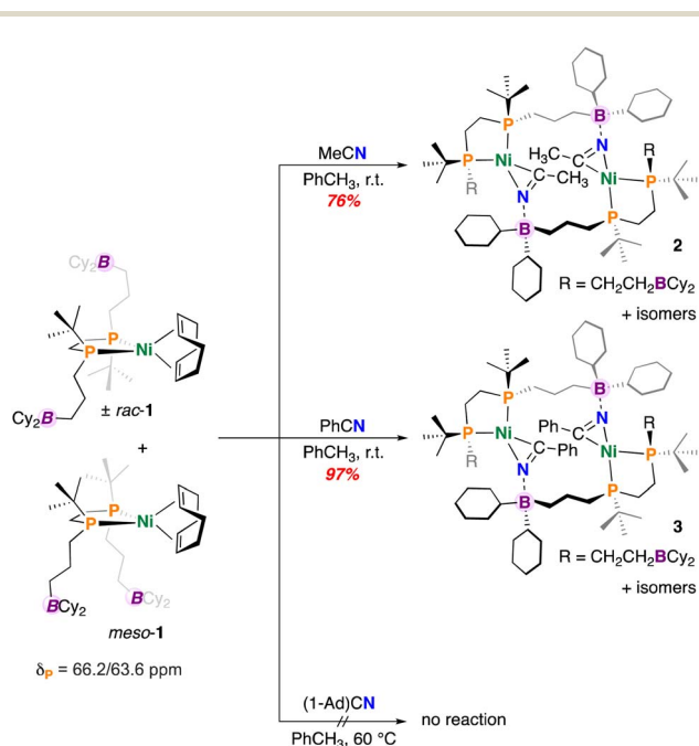
Fig. 2 Synthesis of Ni nitrile complexes.
