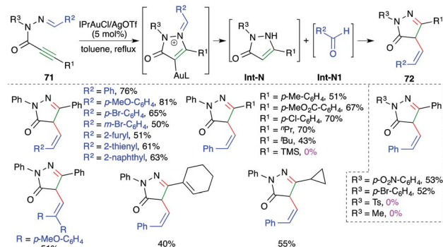
Scheme 46 Synthesis of pyrazolidin-3-ones using intramolecular carboamination.
