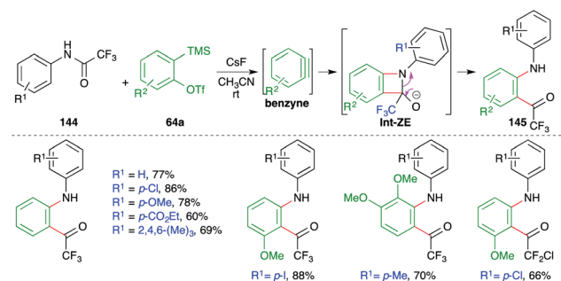
Scheme 79 Metal-free carboamination of benzynes.
