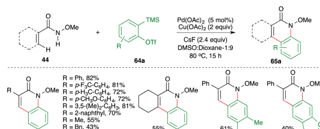
Scheme 42 Synthesis of N -methoxy isoquinolones using the carboamination of benzynes.
