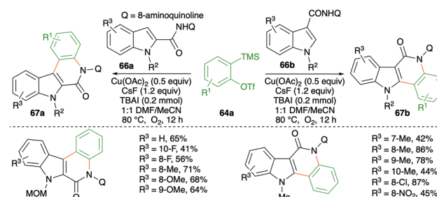
Scheme 43 Synthesis of indole-fused isoquinolones using the carboamination of benzynes.
