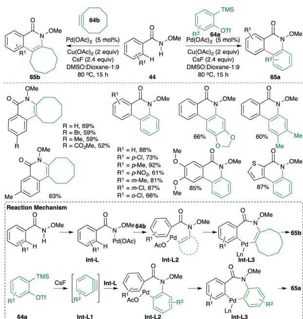
Scheme 41 Carboamination of benzynes with amides.
