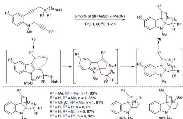
Scheme 48 A carboamination-Friedel-Crafts alkylation-intramolecular cyclization cascade.
