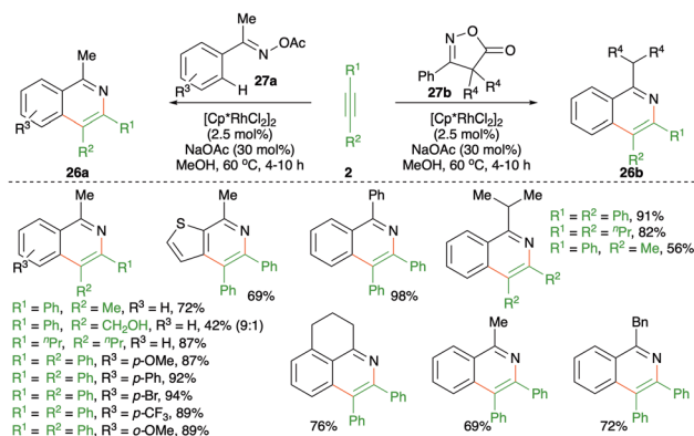
Scheme 15 Carboamination of alkynes with imines and oxazoles.
