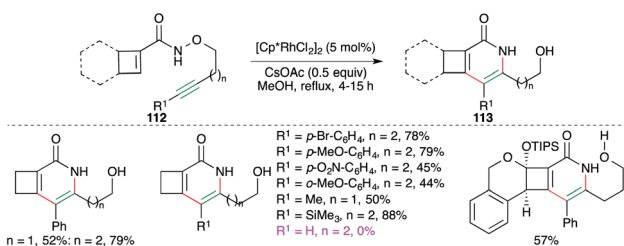
Scheme 64 Tandem carboamination and N–O bond cleavage.
