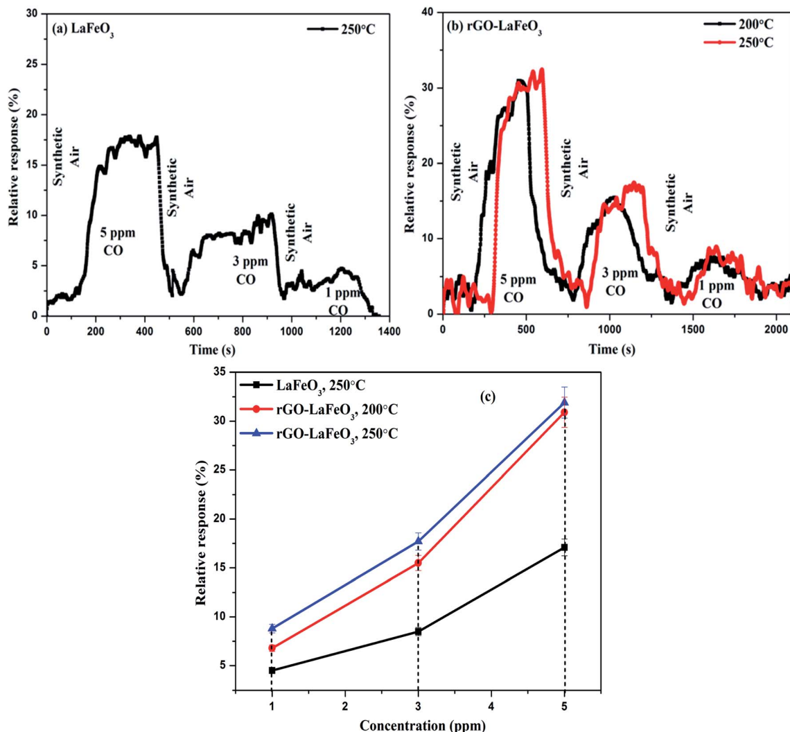
Fig. 13 Relative response with respect to time for LaFeO 3 (a) and rGO-LaFeO 3 (b) and relative response with respect to concentration for LaFeO 3 and rGO-LaFeO 3 (c) towards CO gas at temperatures of 200 and 250 °C.
