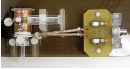
FIGURE 2: The RF coil and transceiver.
