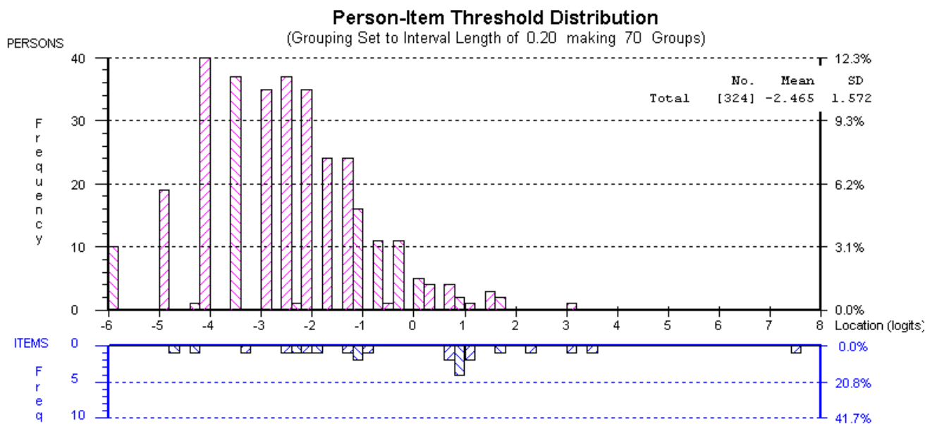
Figure 4 Targeting map for 8-item EPDS.
