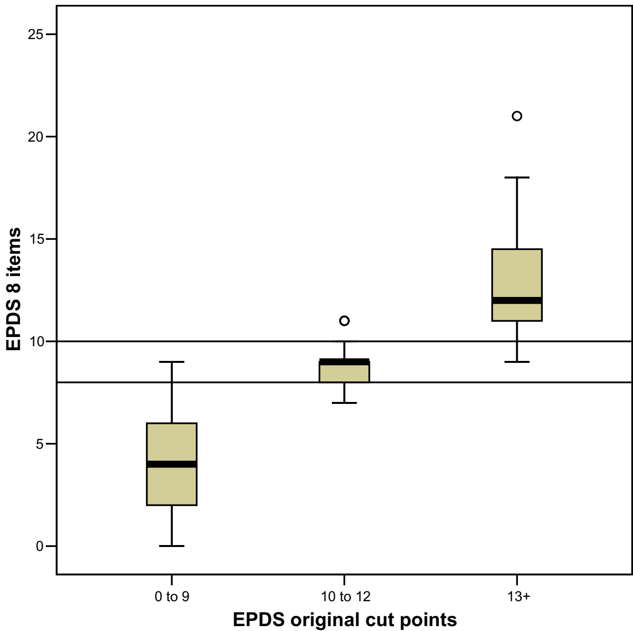
Figure 5 Boxplot showing 8-item EPDS scores for women classified into groups using the original EPDS cutpoints (scores 0 to 9, 10 to 12, 13+).
