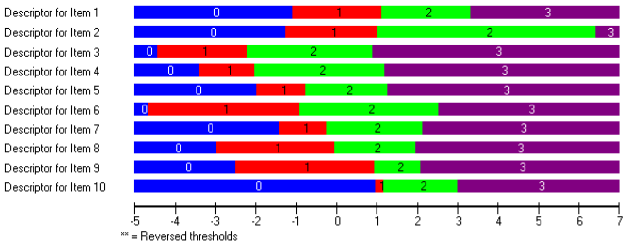
Figure 1 Threshold Map for 10-item EPDS.
