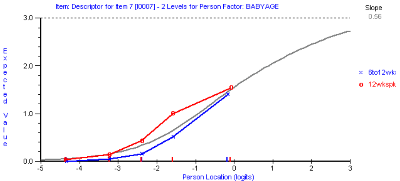
Figure 3 Differential item functioning for age of baby for Item 7.
