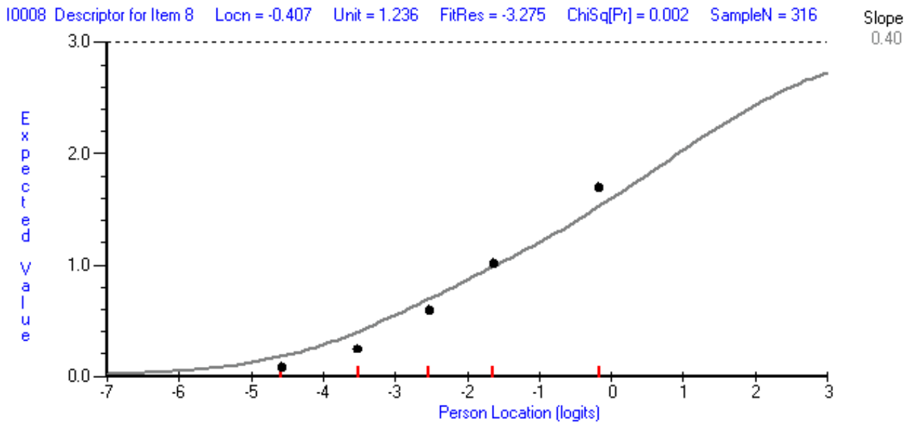
Figure 2 Fit of item 8 I have felt sad or miserable.
