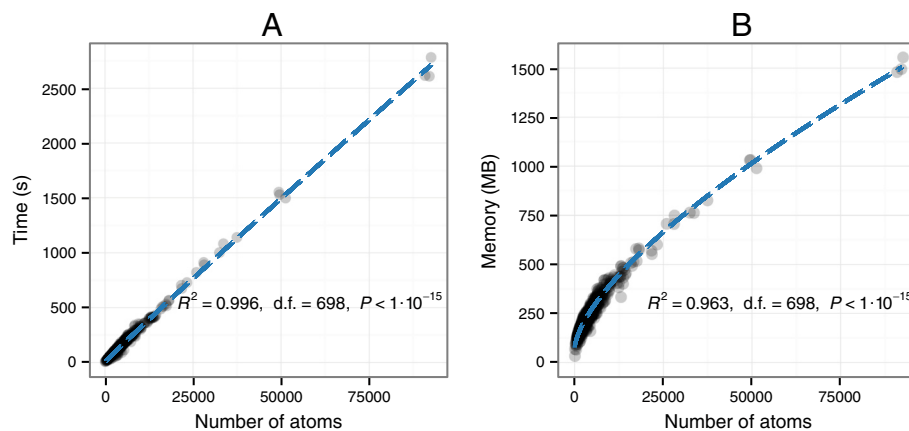
Fig. 3 Execution time (a) and memory consumption (b) of Structuprint, as a function of the atom count (n). The runtime complexity is O(n) , whereas the memory complexity is O(\sqrt{n}) . The uneven distribution of atom counts reflects the composition of the Protein Data Bank. As of March 2015, ~99 % of entries in the PDB had an atom count of 61,000 or less, with the overall mean being 9,006 atoms
