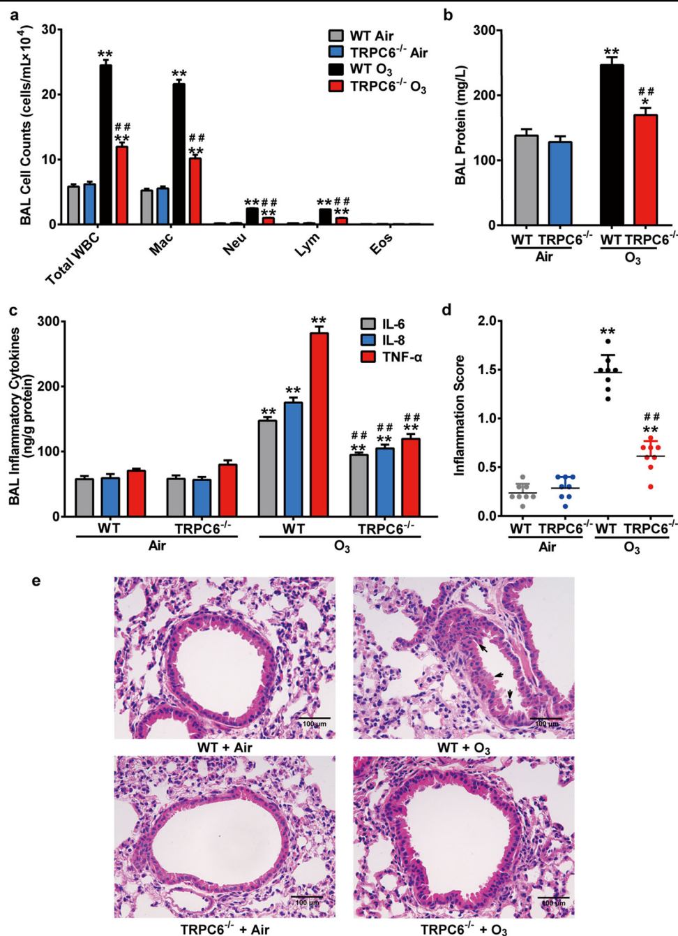
Fig. 1 Effect of TRPC6-deficiency on O 3 -induced airway inflammation. WT and TRPC6 -/- mice were exposed to O 3 (1 ppm) for 3 h every other day (day 1, 3, 5). The mice were anesthetized 24 h after the last exposure. a–c Total white blood cell counts (Total WBC), macrophage counts (Mac), neutrophil counts (Neu), lymphocyte counts (Lym), eosinophil counts (Eos) ( a ), total protein content ( b ) and the release of inflammatory mediators IL-6, IL-8, TNF- \alpha ( c ) in BAL fluid of different groups were compared. d Inflammation scores in air control and O 3 -exposed mice. e Representative histological sections of mouse lungs (H&E staining) after exposure to O 3 or air. Black arrows: inflammatory changes. Scale bar: 100 \mu m. Results are presented as mean \pm SEM, n = 8 . * P < 0.05 or ** P < 0.01 compared with WT + Air group, ## P < 0.01 compared with WT + O 3 group.
