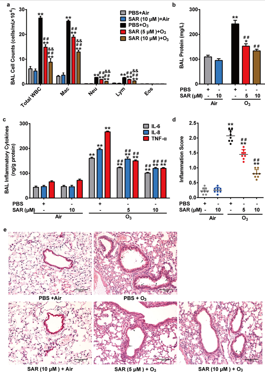
Fig. 2 Effect of TRPC6-blockage on O 3 -induced airway inflammation in mice. WT mice were exposed to O 3 (1 ppm) for 3 h every other day (day 1, 3, 5). Mice received PBS or SAR7334 by oral gavage 4 h before exposure. The mice were anesthetized 24 h after the last exposure. a–c Total white blood cell counts (Total WBC), macrophage counts (Mac), neutrophil counts (Neu), lymphocyte counts (Lym), eosinophil counts (Eos) ( a ), total protein content ( b ) and the release of inflammatory mediators IL-6, IL-8, TNF- \alpha ( c ) in BAL fluid of different groups were compared. d Inflammation scores in air control and O 3 -exposed mice. e Representative histological sections of mouse lungs (H&E staining) after exposure to O 3 or air. Black arrows: inflammatory changes. Scale bar: 100 \mu m. Results are presented as mean \pm SEM, n = 8 . * P < 0.05 or ** P < 0.01 compared with PBS + Air group, ## P < 0.01 compared with PBS + O 3 group, && P < 0.01 compared with SAR (5 \mu M) + O 3 group.
