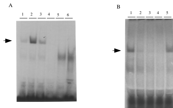
Fig. 2: Gel mobility shift analysis using the -66 to -35 region of \beta CaM kinase II. Ten \mu g of nuclear extract and 0.2 ng of ^{32} P-labeled probe (about 1 \times 10^4 cpm) were used in the experiments. A , tissue specificity of DNA binding protein, Lanes 1 - 6, nuclear extract from forebrain, cerebellum, brainstem, liver, kidney and spleen of rat, respectively. B , specificity of probe. Nuclear extract of cerebellum was incubated with ^{32} P-labeled probe in the presence of non-radioactive probe or competitor DNA. Lane 1, without non-radioactive probe; lanes 2 - 4, in the presence of a 1-, 2.5-, and 5-fold mole excess of non-radioactive probe, respectively; lane 5, in the presence of a 5-fold mole excess of the scrambled sequence.
