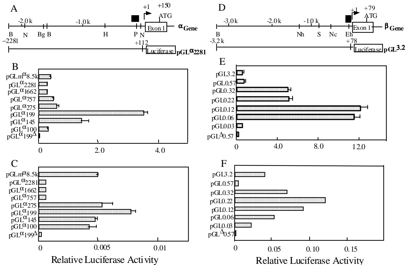
Fig. 1: Promoter-luciferase reporter and deletion analysis of CaM kinase II promoter activity in transiently transfected neuronal and non-neuronal cells. A. A schematic representation of the 5' flanking region of the \alpha CaM kinase II gene (Upper) and one of the \alpha CaM kinase II promoter-luciferase reporters (Lower). \alpha CaM kinase II promoter-luciferase reporters were created by PCR amplification using the 5' flanking sequence of the gene. The sequence is numbered with respect to the transcription initiation site (indicated as +1) shown by an arrow. The box represents exon 1 and the translation initiation site is shown by ATG and +150. Black box shows neuronal cell type-specific promoter region found in this study. Restriction enzyme sites and their positions are shown; B, BamHI; Bg, BglII; H, HindIII; N, NcoI; P, PstI. B and C. Deletion analysis of \alpha CaM kinase II promoter activity in transiently transfected neuronal and non-neuronal cells. Luciferase reporters were co-transfected with the internal control of pcDNA3/ \beta -gal into neuronal cells, NG108-15 ( B ), and into non-neuronal cells, BALB/c3T3 ( C ). Luciferase activity was measured 24 hr later, and is expressed relative to that obtained with the control vector after correcting for the transfection efficiency based on co-transfection with pcDNA3/ \beta -gal. The activity observed with pGL3-control vector was used as a positive control and expressed as 1.00. All values are presented as the mean of three assays. The data are representative of three independent experiments. D. A schematic representation of the 5' flanking region of the \beta CaM kinase II gene (Upper) and one of the \beta CaM kinase II promoter-luciferase reporters (Lower). \beta CaM kinase II promoter-luciferase reporters were created by PCR. The sequence is numbered as in A . Black box shows neuronal cell type-specific promoter region found in this study. Restriction enzyme sites and their positions are shown; B, BamHI; Eh, EhoI; Nc, NcoI; Nh, NheI; S, Sac I. E and F. Deletion analysis of \beta CaM kinase II promoter activity in transiently transfected cells. Luciferase reporters were co-transfected with the internal control of pcDNA3/ \beta -gal to neuronal cells, NG108-15 ( E ), and non-neuronal cells, BALB/c3T3 ( F ). Activity observed with pGL2-control vector was used as a positive control and expressed as 1.00. Luciferase activity was measured after 24 h. Data are representative of three experiments and similar results were obtained.
