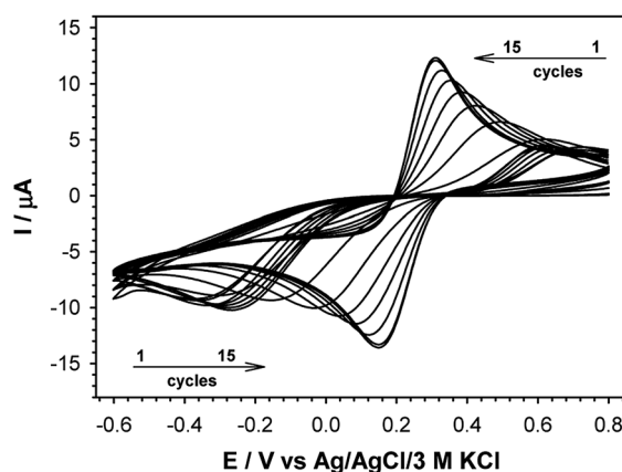
Fig. 4 Subsequent cyclic voltammograms obtained with gold disc electrode modified with 8-mercaptopropionic acid. 5 mM \text{Fe}(\text{CN})_6^{3-} in 0.1 M phosphate buffer containing 150 mM \text{K}_2\text{SO}_4 , pH 7.0, scan rate 0.05 \text{ V s}^{-1} . Thiol layers were formed in 1 mM thiol ethanolic and aqueous solutions.
