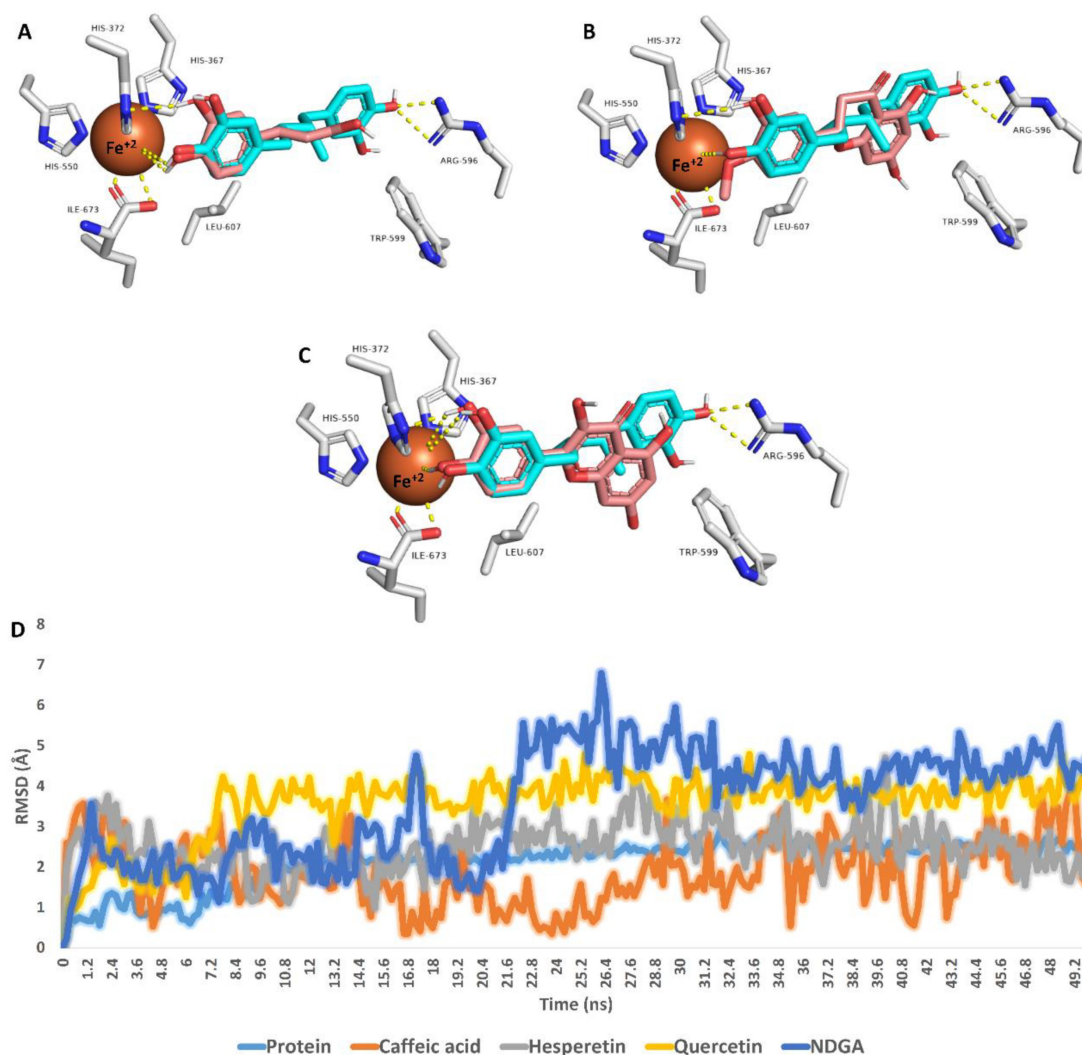
Figure 5. Binding modes of caffeic acid, hesperetin, and quercetin inside the active site of 5-LOX (brick red-colored structures; (A–C), respectively). Each structure with found to be aligned with NDGA (cyan-colored structure), the reported 5-LOX co-crystallized inhibitor, at their catechol moiety. These binding modes were extracted from the MDS runs as the most populated poses. D is the RMSD of each structure inside the 5-LOX active site over 50 ns long MDS.
