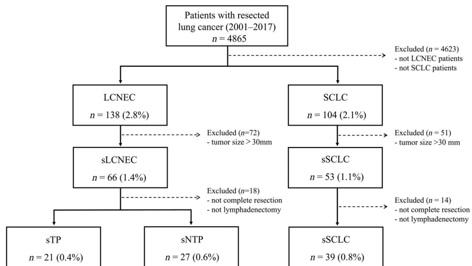
Figure 1 Flow diagram of patients with LCNEC and SCLC in this study. LCNEC, pulmonary large cell neuroendocrine carcinoma; SCLC, small cell lung carcinoma; sLCNEC, small-sized LCNEC patients; sSCLC, small-sized SCLC patients; sTP, small-sized LCNEC patients who were positive for all three neuroendocrine markers (synaptophysin, chromogranin A, and NCAM); sNTP, small-sized LCNEC patients who were positive for one or two of three neuroendocrine markers.
