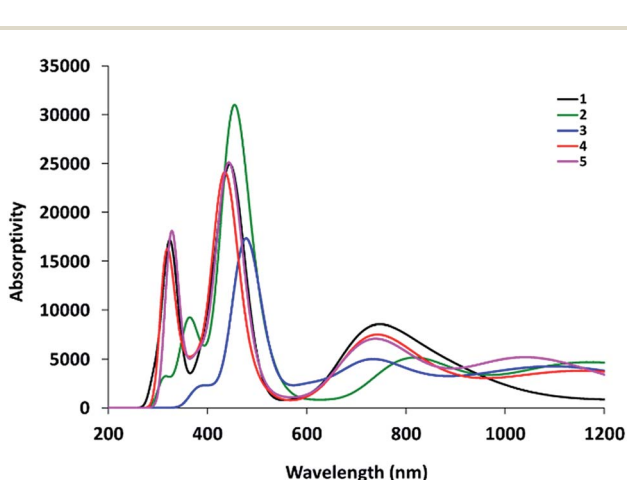
Fig. 7 Triplet-state TD-DFT calculated electronic spectra of 1–5 .
