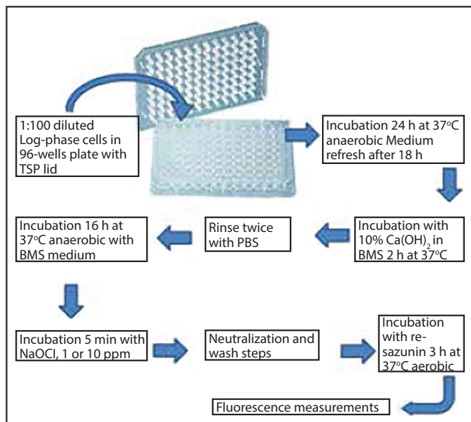
Figure 1. The treatment scheme of the viability assay in which biofilms were exposed to calcium hydroxide (Ca(OH) 2 ) and were subsequently treated with sodium hypochlorite (NaOCl)
