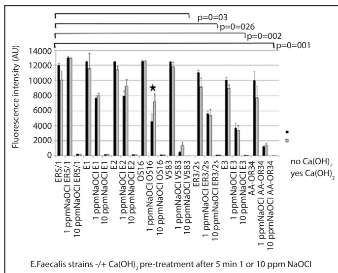
Figure 2. Metabolic activity of various Enterococcus faecalis strains without or with pre-treatment with calcium hydroxide and after a 5-min treatment with 1 or 10 ppm sodium hypochlorite. The controls were treated with phosphate buffered saline. Only one strain, E. faecalis OS16 (marked with a star), became less susceptible to NaOCl after a pretreatment with Ca(OH) 2 (P= 0.03). Error bars represent standard error of the mean. The individual strains are arranged from least susceptible to NaOCl (left) to most susceptible to NaOCl (right). Differences in susceptibility between strains is shown with the bars depicted above the graph
