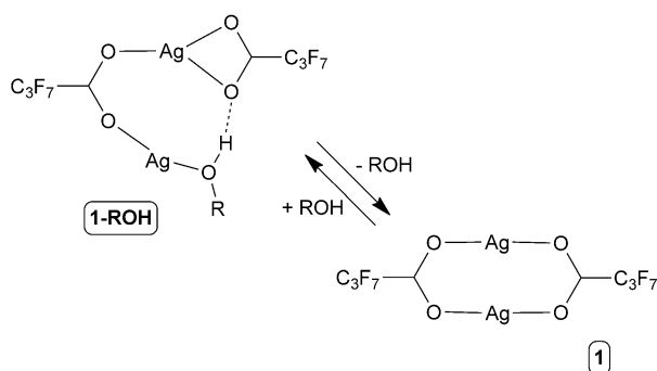
Scheme 1. Reversible alcohol release/uptake by the coordination polymers [\text{Ag}_4(\text{O}_2\text{C}(\text{CF}_2)_2\text{CF}_3)_4(\text{TMP})_3(\text{ROH})_2] ( 1-ROH ; R = Me, Et, i Pr) yielding coordination polymer 1 , here emphasising only the change in carboxylate coordination.
