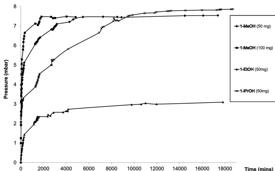
Figure 6. Evolution of the partial pressure of MeOH, EtOH and i PrOH with time.
