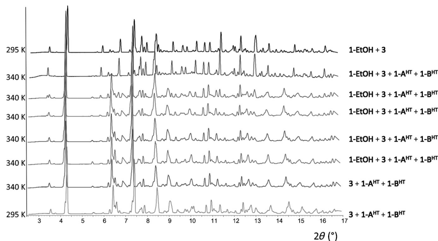
Figure 4. In situ synchrotron powder diffraction study of ethanol release reaction, 1-EtOH → 1-A HT + 1-B HT , at 340 K (from top to bottom). Interval between powder patterns is 20 min. (Compound 3 is an impurity phase that remains unchanged during the conversion of 1-EtOH to 1 ). (Rietveld fits are shown in Figures S7–S14 in the Supporting Information).
