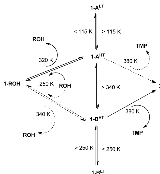
Scheme 4. The proposed reaction manifold showing the conversion 1-ROH \rightarrow [1-A^{HT} \rightleftharpoons 1-B^{HT}] \rightarrow 2 , the first two steps of which are equilibria in a closed environment. There is no definitive experimental evidence for the steps shown with dashed arrows, but the presence of these routes could not be ruled out. The conversions between the four polymorphs of 1, involving changes in temperature, are also indicated.
