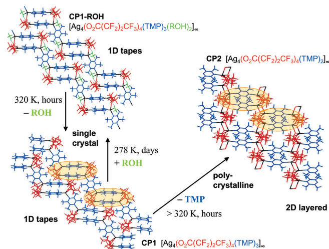
Scheme 2. Reaction scheme showing the relationship between coordination polymers 1-ROH (shown here with R = Me), 1 (as polymorph 1-A HT ) and 2 .
