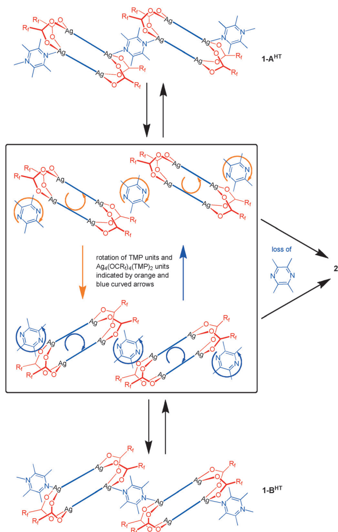
Scheme 3. Proposed mechanism for conversion between polymorphs 1-A^{HT} and 1-B^{HT} involving dissociation of singly-bridging TMP ligands which leads to conversion of 1 \rightarrow 2 by the loss of these dissociated TMP ligands. Conversion between polymorphs 1-A^{HT} and 1-B^{HT} requires no loss of dissociated TMP ligands, but instead requires rotation of these ligands and the residual Ag_4(O_2CR)_4(TMP)_2 units ( R_f = CF_2CF_2CF_3 ) in half of polymers in each crystal. The rotations are indicated by orange and blue curved arrows. The box indicates that the species depicted with dissociated TMP units correspond to a non-isolable intermediate or transition state species in the transformation of 1 \rightarrow 2 .
