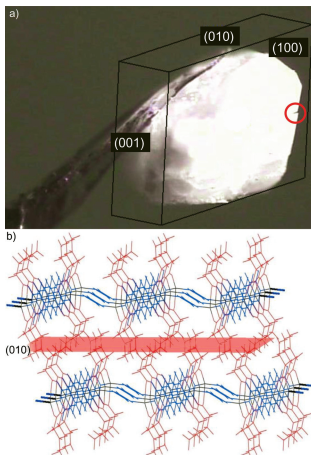
Figure 7. a) Single crystal of 1-A HT (formed by MeOH loss from 1-MeOH) with crystal faces indicated, showing a small crack (circled), which lies parallel to the (010) plane (indexing relative to 1-A HT lattice). b) Crystal structure of 1-A HT view of the perpendicular to the (100) plane with (010) plane shown in red. Colours are as in Scheme 2. Hydrogen atoms not shown.
