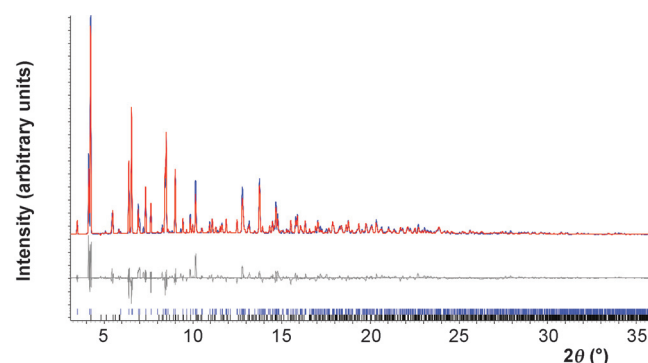
Figure 10. Observed (blue) and calculated (red) profiles and difference plot [ (I_{\text{obs}} - I_{\text{calc}}) ] of the Rietveld refinement for X-ray powder diffraction pattern ( 2 \leq 2\theta \leq 36^\circ , max. resolution 1.33 Å) at 295 K ( R_{\text{wp}} = 0.14769 , R'_{\text{wp}} = 0.30028 gof = 17.132). Composition: 1-B HT (80(1)%) and 2 (20(1)%). Upper tick marks refer to peaks for 1-B HT and lower tick marks refer to peaks for 2 .
