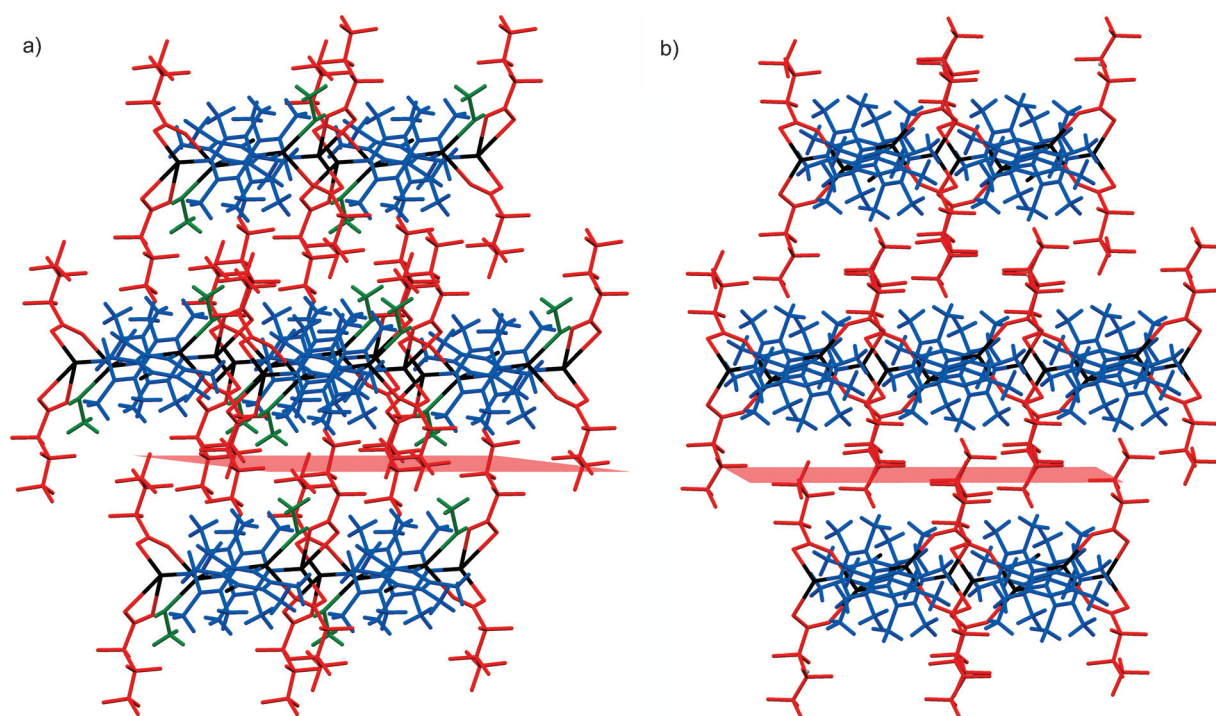
Figure 1. View of a) 1-MeOH and b) 1-A HT along the coordination polymer chains, illustrating the rod-like distorted hexagonal packing motif of these chains. The coordination polymer propagation direction is approximately [113] for 1-MeOH and is [001] for 1-A HT . The (01\bar{1}) planes for 1-MeOH and (010) planes for 1-A HT (shown in red) lie parallel to the fluororous layers. Ag in black, TMP ligands in blue, heptafluorobutanoate in red, methanol in green. Note that lattice indexing is different for the two crystal structures. Alternative views of these structures are shown in Figures 7b and 8b.
