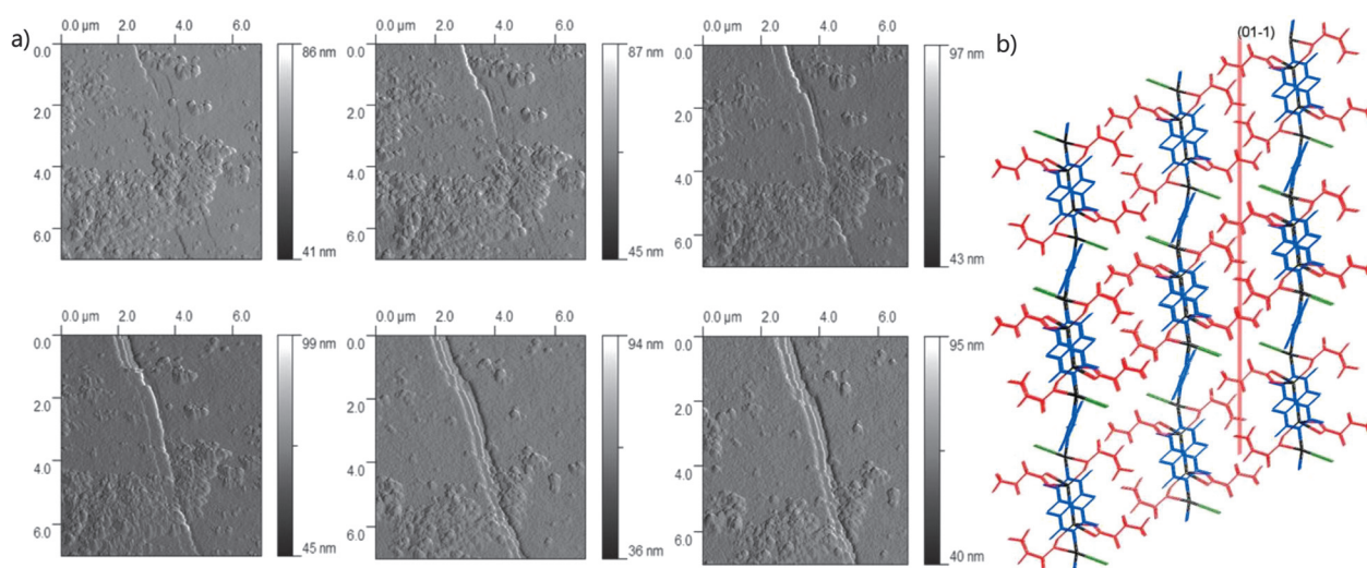
Figure 9. a) Sequence of AFM images of a 7 μm square of the (101) face of a single crystal of 1-MeOH recorded at 308 K in tapping mode at 8 min intervals during the release of MeOH. b) View of the crystal structure of 1-MeOH perpendicular to the (101) face (as for the AFM images) with (011) plane indicated as a red line. Colours as in Scheme 2. Hydrogen atoms not shown.
