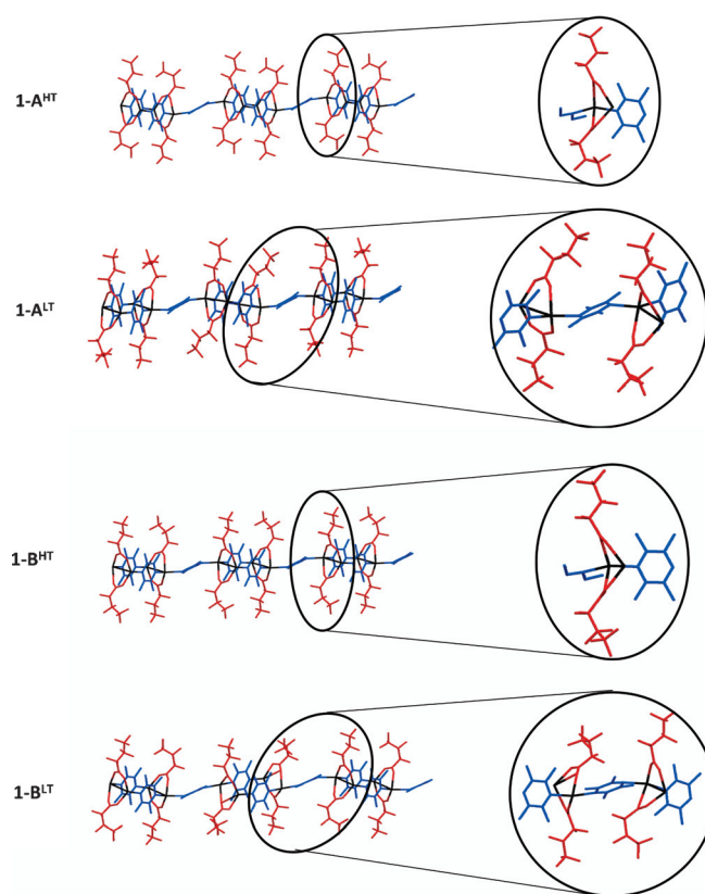
Figure 2. Crystal structures of the four polymorphs ( 1-A HT , 1-A LT , 1-B HT and 1-B LT ) of coordination polymer 1 [Ag 4 (O 2 C(CF 2 ) 2 CF 3 ) 4 (TMP) 2 ]. Expansions show the asymmetric units, highlighting: i) the coordination environment of the Ag I centres; and ii) the different conformational distributions ( gauche:anti ) of the perfluoroalkyl chains. Hydrogen atoms are not shown. In expanded views TMP ligands are only shown in part for polymorphs 1-A HT and 1-B HT . Colour code as in Figure 1.
