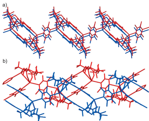
Figure 3. a) Crystal structure of polymorph 1-A HT viewed along the [010] direction showing tapes stacked directly upon each other and b) crystal structure of polymorph 1-B HT viewed along the [001] direction showing tapes that are related by a 2 1 screw axis that lies along the vertical axis of this view (i.e. [010]). Blue and red colours denote adjacent tapes stacked along the viewing direction. Hydrogen atoms not shown.
