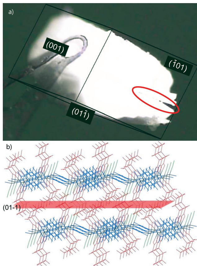
Figure 8. a) Single crystal of crystal 1-MeOH , formed from crystal of 1-A HT after 24 h exposure to MeOH vapour, indicated the enlarged crack (circled), which lies parallel to the (011) planes (indexing relative to 1-MeOH lattice). b) Crystal structure of 1-MeOH viewed perpendicular to the (101) plane with (011) plane shown in red. Colours are as in Scheme 2. Hydrogen atoms not shown.
