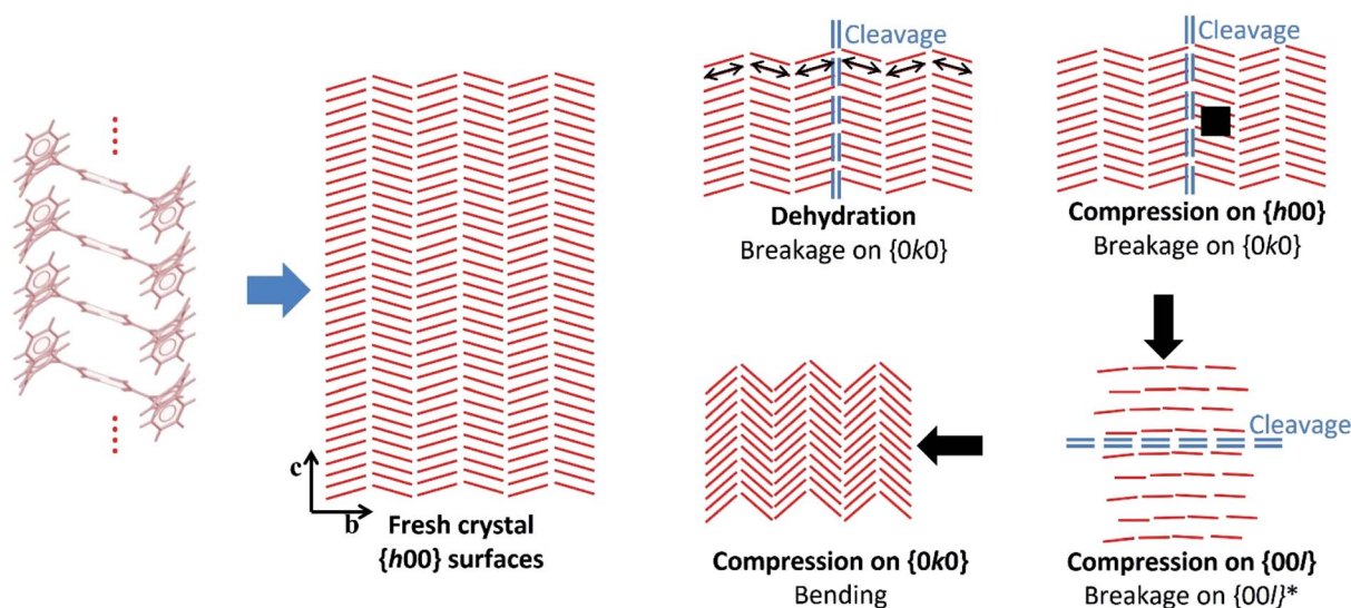
Fig. 6 Scheme illustrating the hypothetical effects of dehydration and compression on the crystals of CBZ·2H 2 O based on the experimental data and the structural analyses. Bending upon compression on {0k0} is hypothesised after Reddy et al. (2005) 35 and Reddy, Padmanabhan & Desiraju (2006). 38 The red lines correspond to the CBZ dimers projected on the {h00} surfaces, and the arrows show the direction of the compressive forces.
