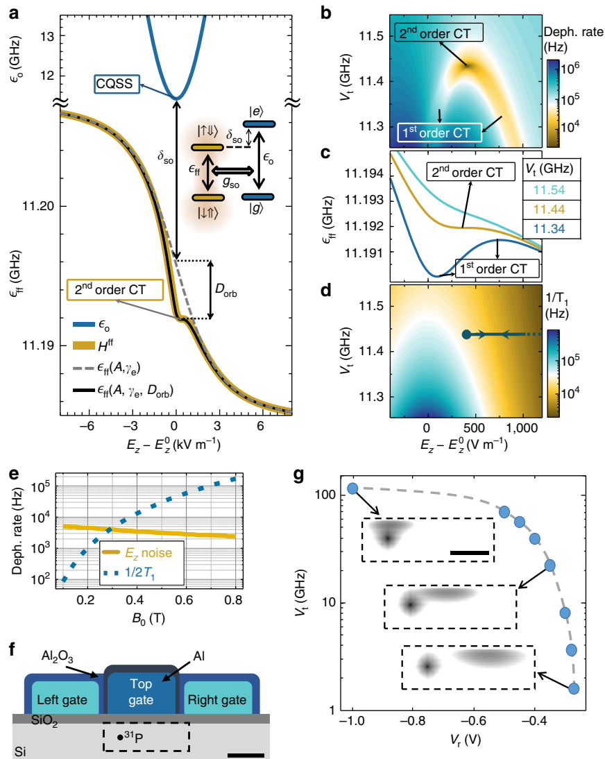
Fig. 2 Robustness to electric noise. a Charge, \epsilon_o , and flip-flop, \epsilon_{ff} , qubit transition frequencies as a function of vertical electric field E_z for B_0 = 0.4 T, A = 117 MHz, d = 15 nm, \Delta_r = -0.2\% and V_t = 11.44 GHz. The inset shows the level diagram of flip-flop states coupled to charge states. CT stands for “clock transition” and CQSS for “charge qubit sweet spot”. b Estimated flip-flop qubit dephasing rate, assuming electric field noise E_{z,noise} = 100 V m ^{-1} . c E_z -dependence of flip-flop precession frequency for the three indicated tunnel coupling values. d Flip-flop qubit relaxation rate, with arrows indicating the adiabatic path used for z-gates. e Flip-flop qubit dephasing rate due to E_z noise and relaxation, at second-order CTs for each B_0 . f Device structure to tune the tunnel coupling V_t of the charge qubit. Scale bar is 30 nm. g V_t as a function of right gate voltage, calculated using a finite element Poisson solver (Synopsis TCAD) and atomistic tight binding (NEMO-3D) 72 . The insets illustrate the NEMO-3D wavefunctions inside dashed region in f , for three right gate voltages V_r = -1, -0.35 and -0.27 V. The left gate voltage is V_l = -0.5 V for all the simulations, and the top gate is biased such that the position of the electron is in between the donor and interface. Scale bar is 20 nm. The donor is assumed to be z_d = 9.2 nm below the Si/SiO _2 interface
