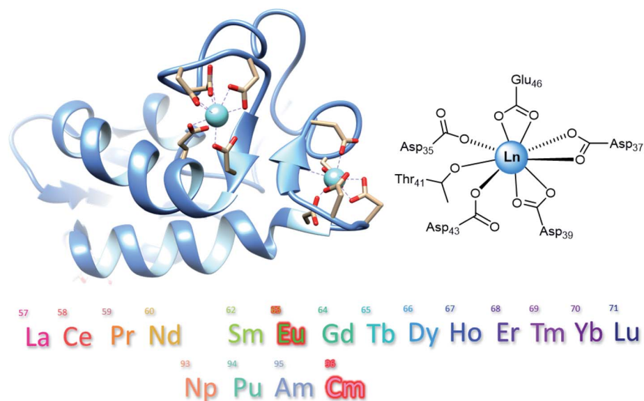
Fig. 1 NMR-determined structure of Y 3+ -LanM with two of the high-affinity EF hands shown in more detail and close-up view of EF1. Below the Ln and An that were used to investigate inter-metal competition of LanM. Eu 3+ and Cm 3+ were used as luminescence probes.
