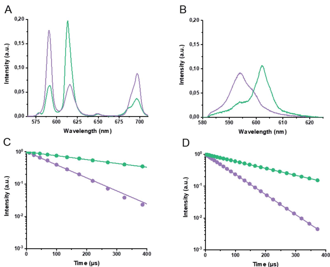
Fig. 2 (A) Deconvoluted Eu 3+ -LanM and Eu 3+ -aquo ion emission spectra from TRFES data. (B) Deconvoluted Cm 3+ -LanM and Cm 3+ -aquo ion emission spectra from TRFES data. (C) Luminescence decays with lifetime fits of Eu 3+ species. (D) Luminescence decays with lifetime fits of Cm 3+ species. Data of the Ln-/An-aquo ions shown in purple and LanM complexes in green. For studies with Eu 3+ , an excitation wavelength of 394 nm was chosen while for Cm 3+ titrations 396 nm was selected. Concentrations of 1 μM LanM and 5.5 μM Eu 3+ or 18 nM LanM and 100 nM Cm 3+ were used for the measurements.
