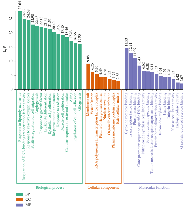
FIGURE 4: GO function enrichment results of SZRD in the treatment of PDSD.
