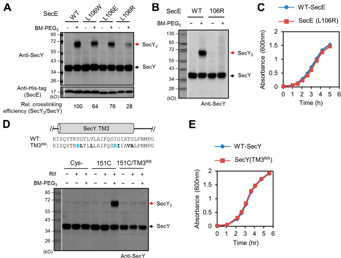
Figure 6. Mutants disrupting the association of SecY complexes in the membrane. (A) The back-to-back association of SecY complexes was tested using a cysteine at position 212 and the bi-functional cross-linker bismaleimide-PEG 3 (BM-PEG 3 ). Mutations were introduced at position 106 of SecE to test their effect on SecY dimer (SecY 2 ) formation. The samples were analyzed by SDS-PAGE and immunoblotting for SecY and His tag (SecE). The cross-linking efficiency was quantitated and is expressed relative to that with wild-type SecE. (B) As in A, but with the chromosomal SecE copy deleted. (C) The growth rate of the cells used in B was compared. The data shown are from a single representative experiment out of two repeats. (D) The front-to-front association of SecY complexes was tested using a cysteine at position 151 and the bi-functional cross-linker bismaleimide-PEG 3 (BM-PEG 3 ). Mutations were introduced in TM3 of SecY, as indicated (TM3 RR ), to disrupt SecY dimer (SecY 2 ) formation. Where indicated, cells were treated with rifampicin (Rif) before cross-linking. (E) The growth rate of the cells used in D was compared. The data shown are from a single representative experiment out of two repeats.
