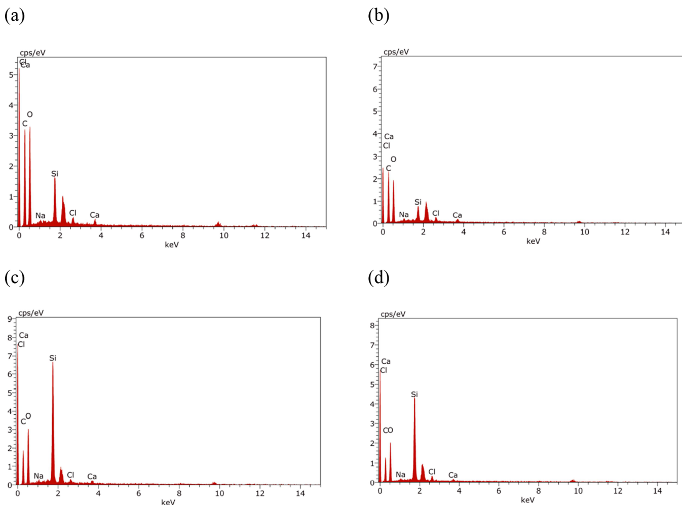
Figure 10. EDX analysis of cellulose isolated from date palm leaves: (a) Cellulose 1, (b) Cellulose 2, (c) Cellulose 3, and (d) Cellulose 4.
