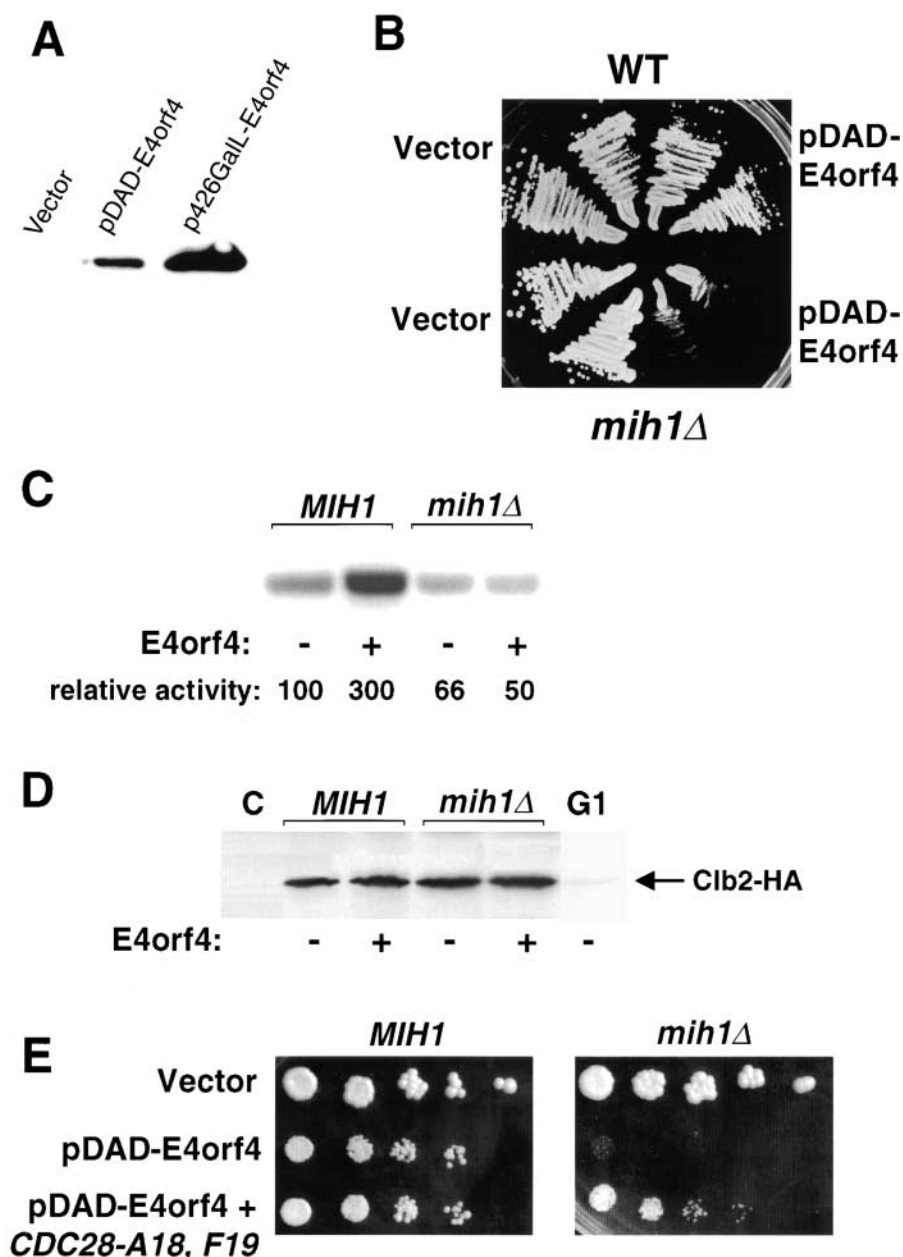
Figure 5. Functional interaction of E4orf4 with Mih1. (A) To compare E4orf4 expression levels from the pDAD and p426-Gall vectors, cells were induced with galactose for 3 h, and E4orf4 levels were determined by Western blot. (B) Wild-type or mih1 Δ cells carrying the indicated plasmids were grown on galactose plates for 2 d. (C) KY630 ( MIH1 ) or KY631 ( mih1 Δ) cells carrying a CLB2-3xHA construct integrated at CLB2 and transformed with either vector or p426Gall-E4orf4 were induced for 6 h with galactose. Clb2-associated kinase activity in the extracts was determined using Histone H1 as substrate. The amount of Histone H1 phosphorylation was measured with a phosphorimager. (D) Clb2-3xHA levels in the extracts described in C were determined by Western blotting. C, a no tag control; G1, an extract of CLB2-3xHA -expressing mutant cells arrested at restrictive temperature in G1. (E) MIH1 and mih1 Δ cells were transformed with the indicated plasmids, and serial dilutions were plated dropwise on galactose plates.
