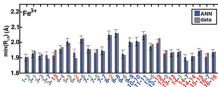
Fig. 10 ANN model predictions (ANN, blue bars) and computed (data, gray bars) minimum LS Fe 3+ bond lengths, \min(R_{LS}) , in Å. Complexes are labeled as equatorial and then axial ligands according to the numbering indicated in Fig. 1 and color-coded by direct ligand atom (green for chlorine, gray for carbon, blue for nitrogen, and red for oxygen). The error bars represent an estimated \pm 1 standard deviation credible interval around the mean prediction, and error bars that do not encompass the computed value are highlighted in red. Fe(III)(Cl) 6 (1-1) is excluded due to being off scale: it has a predicted/calculated bond length of 2.44/2.45 Å, and an error standard deviation of \pm 0.02 .
