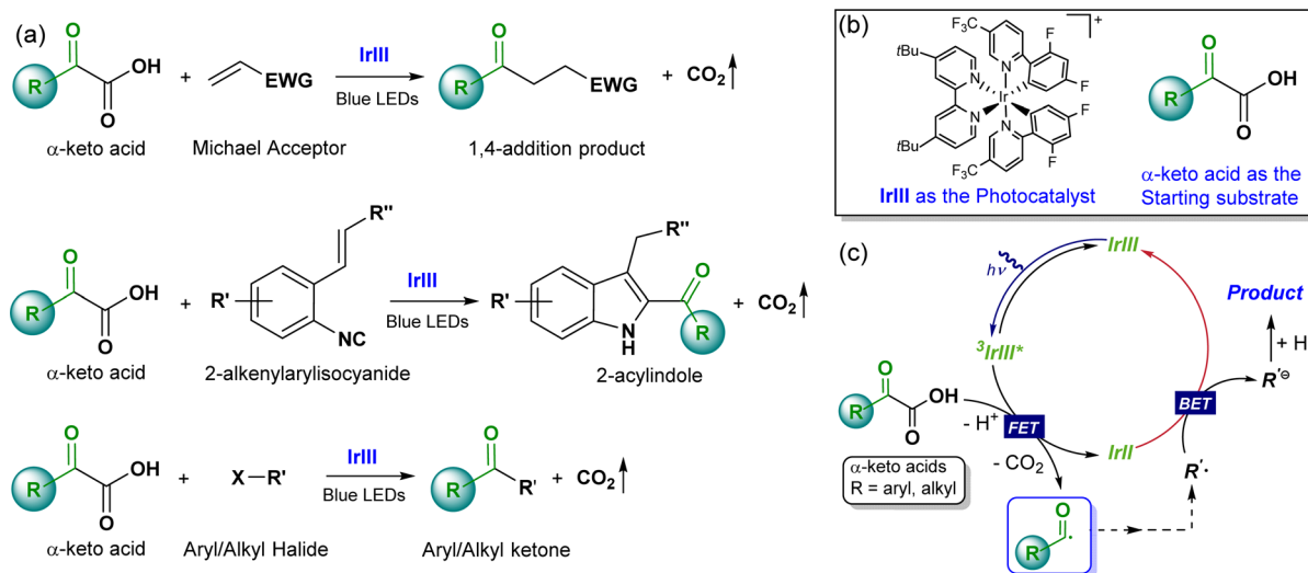
Scheme 1 (a) Novel [\text{Ir}(\text{dFCF}_3\text{ppy})_2(\text{dtbbpy})]^+ ( IrIII ) photocatalytic radical acylation reactions; (b) structures of IrIII and \alpha\text{-keto acid} ; (c) previously proposed photoredox catalytic mechanism with a single-photon cycle.
