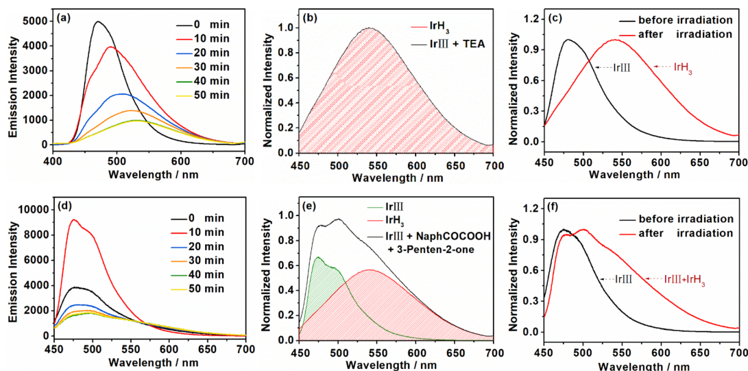
Fig. 3 (a) Steady-state emission spectra of IrIII (150 \mu M) + TEA (50 mM) under deoxygenated conditions in ACN/phosphate buffer (pH 7, v/v = 1 : 1) under continuous illumination by 430 nm laser (20 mJ); (b) species analysis of IrIII + TEA; (c) steady-state emission spectra of IrIII + TEA before (black) and after (red) 40 min continuous illumination by 430 nm laser (20 mJ). (d) IrIII (150 \mu M) + NaphCOCOOH (10 mM) + 3-pentyl-2-ketone (100 mM) under deoxygenated conditions in ACN/phosphate buffer (pH 7, v/v = 1 : 1) under continuous illumination by 430 nm laser (20 mJ); (e) species analysis of IrIII + NaphCOCOOH + 3-pentyl-2-ketone; (f) steady-state emission spectra of IrIII + NaphCOCOOH + 3-pentyl-2-ketone before (black) and after (red) 40 min continuous illumination by 430 nm laser (20 mJ).
