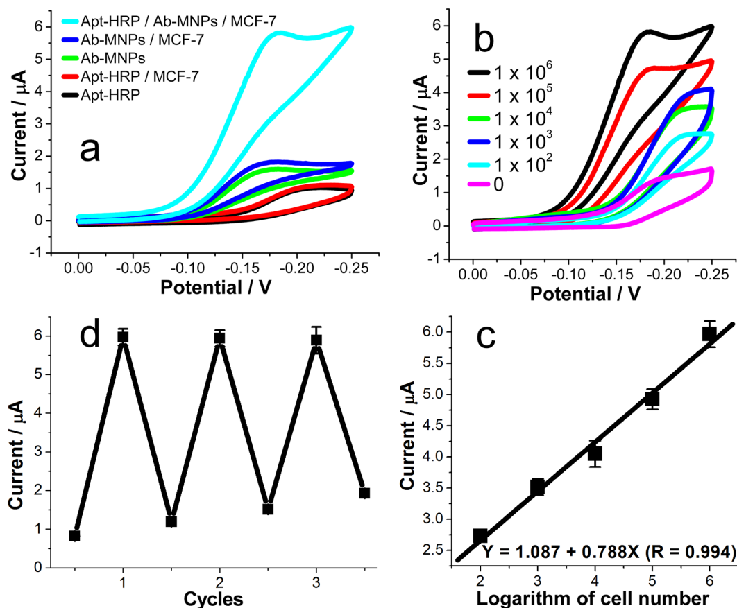
Figure 5 | Cyclic voltammetric responses of (a) the complete (cyan curve) or incomplete (black, red, green, and blue curves) MCMA in the electrolyte containing 20 \mu M thionine and 6 mM H_2O_2 and (b) the MCMA fabricated with different amounts of cells. Other conditions were the same as those in (a). (c) The relationship between the peak current and the cell numbers. The dots represent the currents of the corresponding cyclic voltammogram at -0.25 V. (d) The current response for the MCMA with 1 \times 10^6 cells over three cycles. The top dots represent responsive currents, whereas the bottom dots represent background currents. All dots were taken from the corresponding cyclic voltammogram at -0.25 V.
