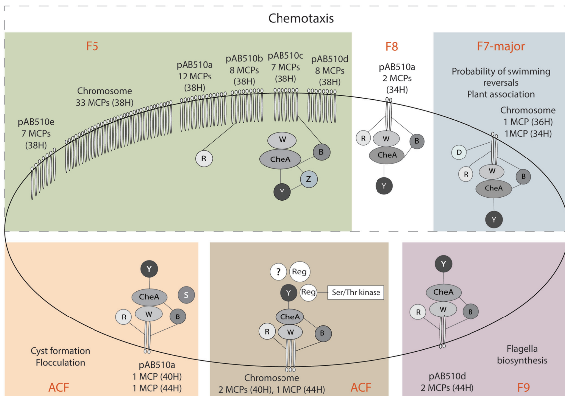
Figure 2. Reconstruction of chemosensory pathways in Azospirillum sp. B510 using the MiST 3.0 database.
