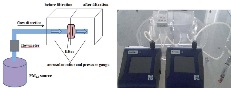
Fig. 2 Schematic diagram and photo-image of the experimental setup for PM 2.5 removal experiment.
