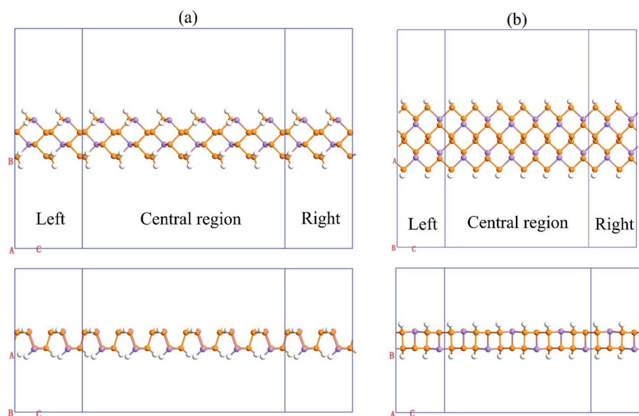
Fig. 10 The schematic diagrams of the structure of (a) armchair device and (b) zigzag device composed of P-I phase (the upper part is the top view and the lower part is the side view), respectively. All one-dimensional devices are saturated by hydrogen atoms, and the ribbon width of the armchair device is 27.64 \text{ \AA} in the transport direction and 7.47 \text{ \AA} perpendicular to the transport direction, the ribbon width of the zigzag device is 19.80 \text{ \AA} in the transport direction and 10.20 \text{ \AA} perpendicular to the transport direction.
