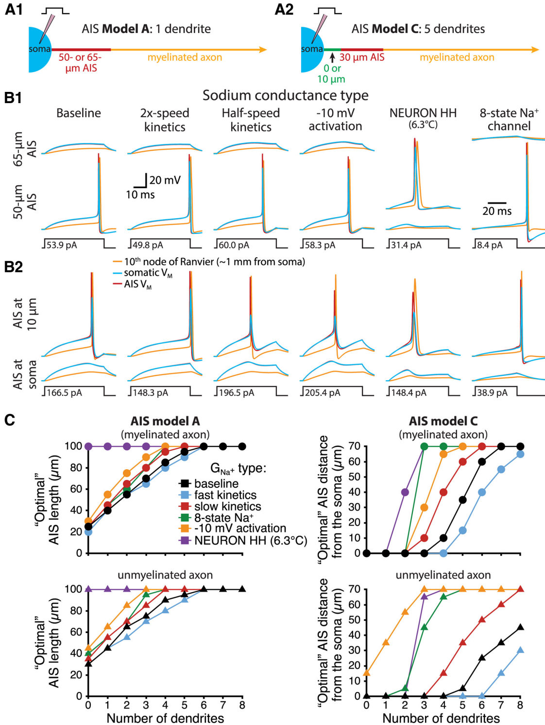
Figure 4. AIS performance across a range of sodium conductance properties. A , Diagrams of the AIS of a one-dendrite myelinated neuron having a 50- or 65- \mu\text{m} -long AIS beginning at the soma ( A 1 ), and of a five-dendrite model with a 30- \mu\text{m} -long AIS beginning either at the soma or 10 \mu\text{m} away ( A 2 ). B , Voltage responses at the soma (blue), AIS (red), or 10th node of Ranvier (~1 mm from the soma; yellow) in response to the indicated current steps in models having the indicated sodium conductance properties and AIS architectures. In most one-dendrite models, increasing AIS length from 50 to 65 \mu\text{m} reduced neuron excitability ( B 1 ), while in the five-dendrite model, moving the 30- \mu\text{m} -long AIS 10 \mu\text{m} away from the soma increased neuron excitability ( B 2 ). C , Comparisons of "optimal" (i.e., lowest rheobase) AIS lengths (left) and locations (right) for myelinated (top) and unmyelinated (bottom) model neurons having the indicated number of dendrites and sodium conductance properties.
