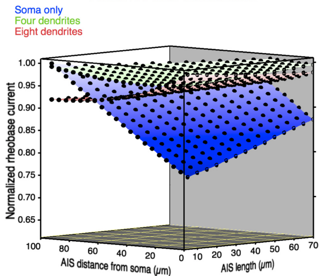
Movie 2. Interaction of AIS length and location in setting neuron excitability in model neurons having conserved total AIS conductances. Shown is a rotating 3-D plot of normalized rheobase currents for each AIS length and location combination for the soma-only model neuron (blue), and neurons with four (green) or eight (red) dendrites in models having conserved (i.e., length-independent) maximal sodium and potassium conductances in the AIS.
