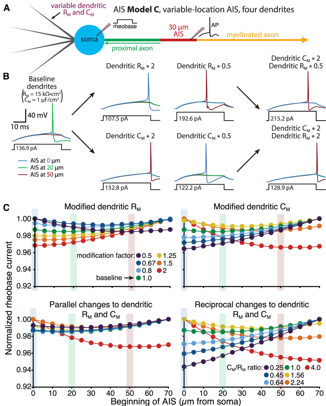
Figure 12. Dendritic membrane properties influence optimal AIS location relative to the soma. A , Diagram of a neuron with four dendrites having variable dendritic membrane properties and a 30 \mu\text{m} AIS positioned at variable distances from the soma (AIS Model C; myelinated axon). B , Voltage responses in the AIS during somatic current injections under baseline conditions (far left) and after manipulations of dendritic R_M and/or C_M , as indicated. Responses from three models are superimposed: those having the AIS beginning 0 (blue), 20 (green), or 50 \mu\text{m} (red) from the soma. C , Plots of normalized rheobase current vs AIS location for the four-dendrite models having modified dendritic R_M (top left), dendritic C_M (top right), parallel changes in both dendritic R_M and C_M (bottom left), or reciprocal changes in dendritic properties (bottom right). Dendritic C_M and/or R_M were multiplied by the indicated modification factors. C_M/R_M ratios in reciprocal manipulations of R_M and C_M are centered around baseline ( C_M/R_M ratio = 1) values. Increasing dendritic C_M and/or dendritic conductance (lower dendritic R_M ) enhanced excitability at more distal AIS locations. Shaded bars indicate the AIS locations for which traces are shown in B .
