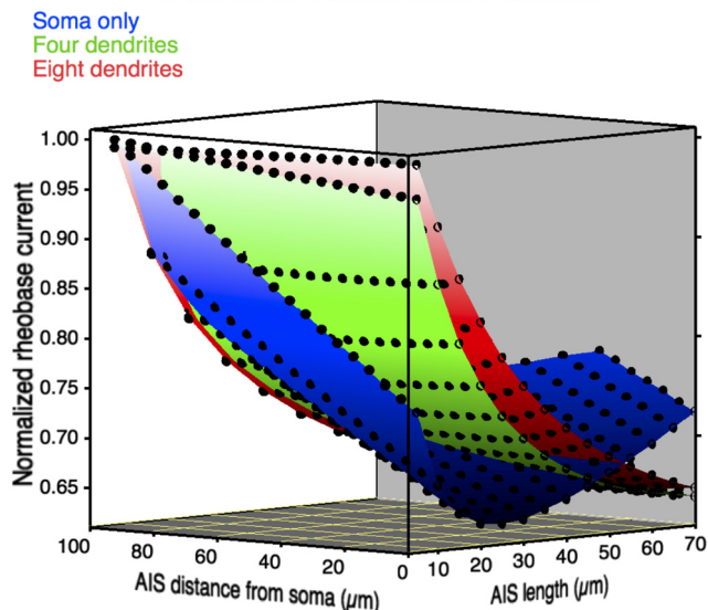
Movie 1. Interaction of AIS length and location in setting neuron excitability in model neurons having conserved conductance densities in the AIS. Shown is a rotating 3-D plot of normalized rheobase currents for each AIS length and location combination for the soma-only model neuron (blue), and neurons with four (green) or eight (red) dendrites in models where the AIS has conserved conductance densities (i.e., total available sodium and potassium conductances increase with AIS length).
