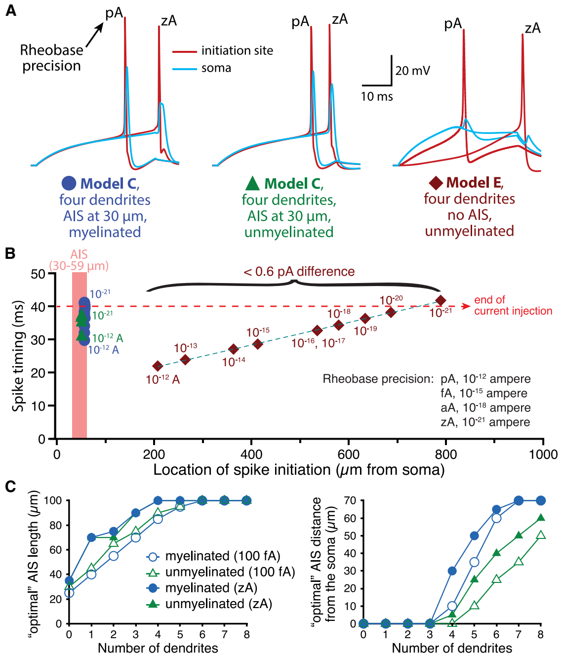
Figure 14. Impact of rheobase precision on action potential initiation and AIS plasticity. A , Plots of action potential waveforms recorded in the AIS (red; 30 μm long and 30 μm from the soma) or in the soma (blue) of neurons with four dendrites and either an AIS associated with a myelinated axon (left), an unmyelinated (middle) axon (AIS Model C), or an unmyelinated axon lacking an AIS (AIS Model E; right). Shown are traces in which rheobase current was calculated to the nearest pA or to the nearest zA, as indicated (simulations used 100 ns time-steps). B , Plots of spike latency vs the location of spike initiation in myelinated and unmyelinated neurons having an AIS (Model C), or in a neuron lacking an AIS (Model E), for rheobase current injections at the indicated precision levels (i.e., rounded up to the nearest suprathreshold stated unit). Note that approaching ever more precise rheobase currents increased the latency to spike initiation and, in the absence of an AIS, moved the location of initiation to very distal regions of the axon. C , Plots of AIS lengths (left) or locations (right) having the lowest rheobase currents, as determined to the nearest 100 fA (open symbols) or 1 zA (closed symbols) in myelinated and unmyelinated neurons.
