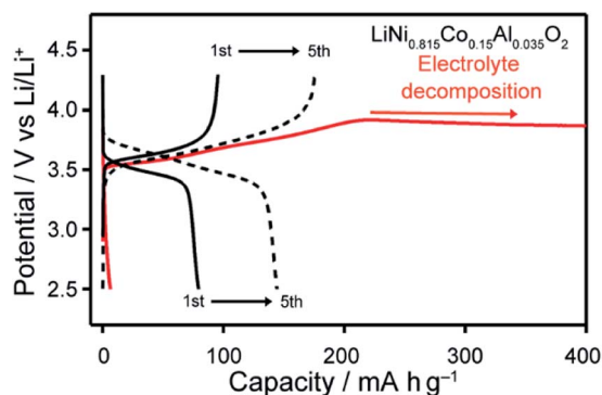
Fig. 9 Charge-discharge curves of Li half-cells composed of LC electrolytes of 1/LiTFSI (black) and 3/LiTFSI (red), and \text{LiNi}_{0.815}\text{Co}_{0.15}\text{Al}_{0.035}\text{O}_2 , recorded at 80 °C.
