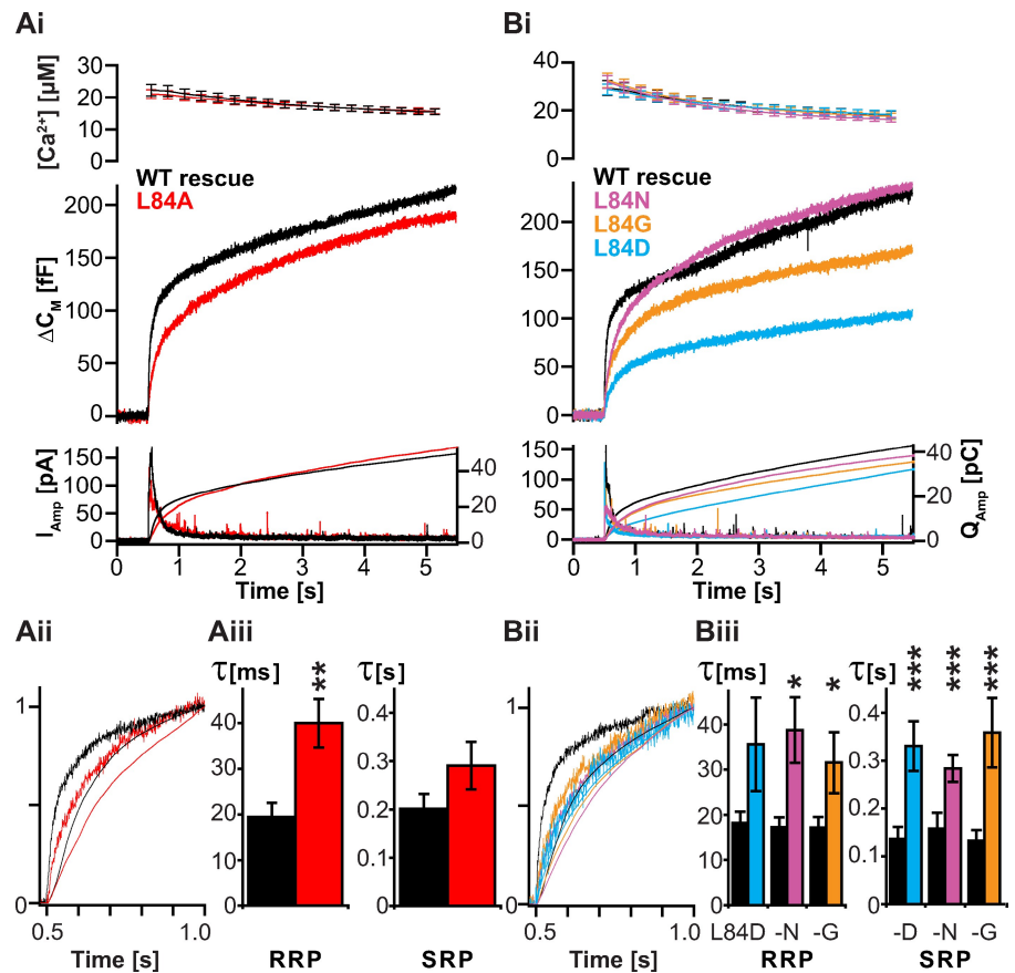
Figure 5. C-terminal mutants of syb-2 cause a slowdown of transmitter release. The C-terminal mutants of syb-2 are shown in Fig. 1. (Ai and Bi) Mean secretion in flash-evoked transmitter release is slowed down. (Aii and Bii) Detailed views of normalized traces in Ai and Bi show that the kinetics of release are slowed down in all cases. (Aiii and Biii) Time constants of the RRP and SRP obtained by fitting of exponentials show slowdown of release in the L84A mutant (Aiii: control, n = 19 ; and L84A, n = 25 ) and L84N, L84G, and L84D mutations (Biii: control, n > 15 ; L84D, n = 9/14 ; L84G, n = 13/17 ; and L84N, n = 15/19 for RRP/SRP time constants; and *, P < 0.05 ; **, P < 0.01 ; and ***, P < 0.001 in t test). (Ai, Aiii, Bi, and Biii) Mean \pm SEM is shown.
