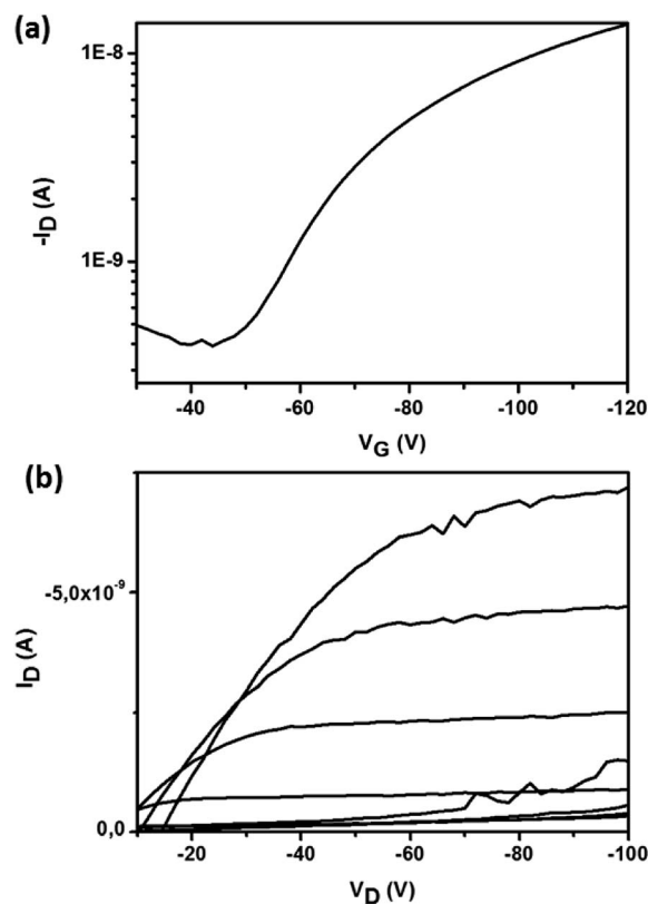
Fig. 6 (a) Transfer (at a fixed V_{\text{D}} value of 100 V) and (b) output plots ( V_{\text{G}} was varied from 20 V to -120 V) for compound Bzt-tpa for hole transport.
