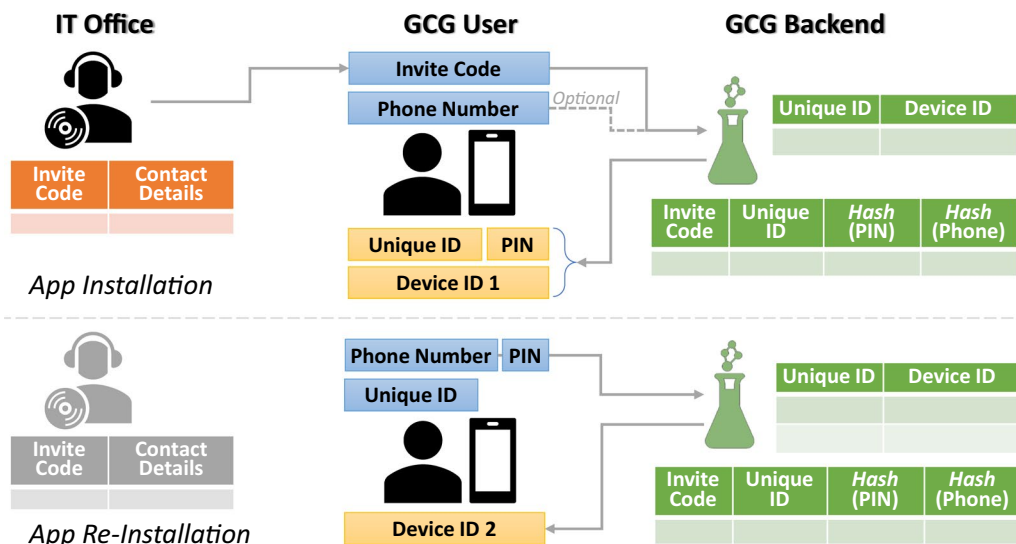
Figure 2: Identifier mapping during GCG App installation.
