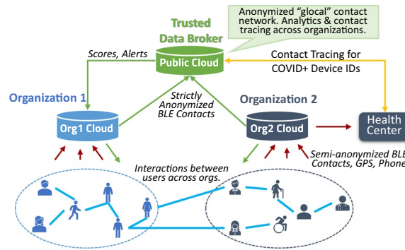
Figure 11: Federated deployment of GCG across Institutions.
