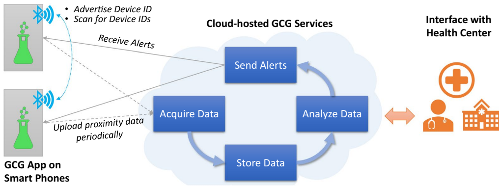
Figure 1: Overall Design of GCG.
