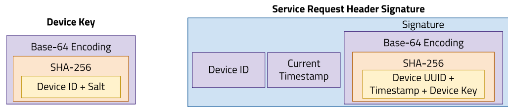
Figure 5: Signing service requests using device key.
