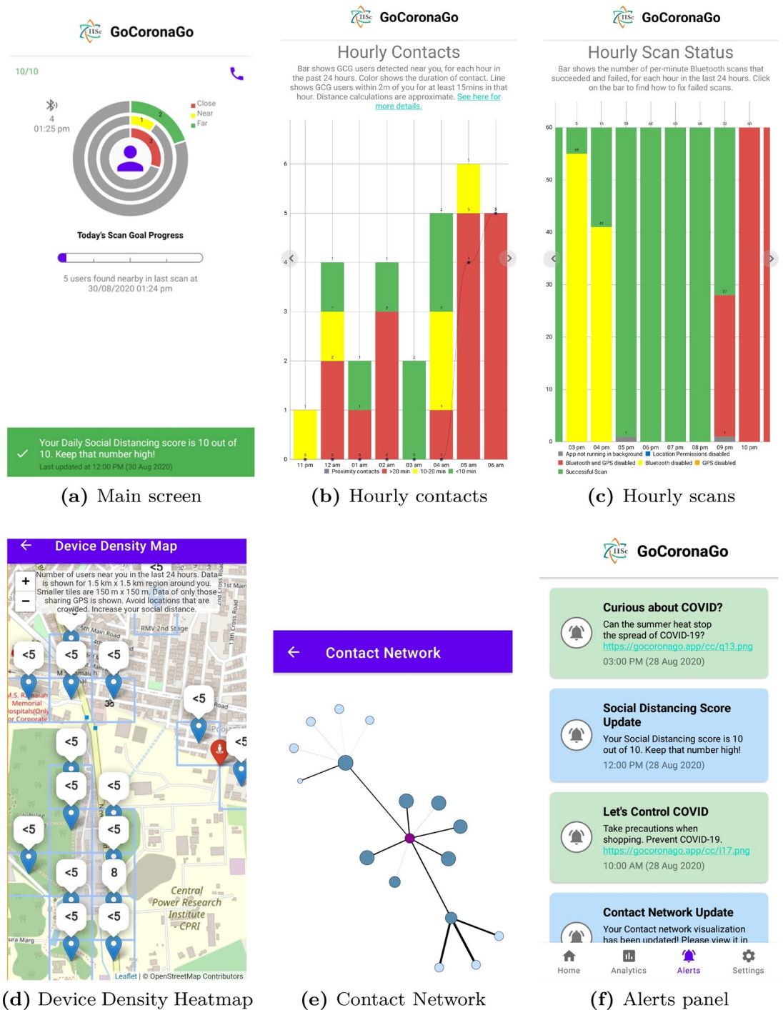
Figure 3: User interface and analytics in the GoCoronaGo v0.7 Android App.
