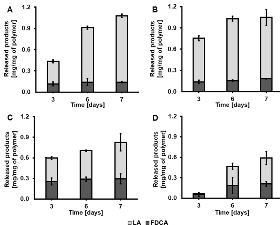
Figure 5. HPLC analysis of acids released from PLA/PPeF blends and the P(LA50PpE50) copolymer. Dark gray bars: 2,5-furandicarboxylic acid (FDCA); light gray bars: lactic acid (LA). (A) PP20; (B) PP30; (C) PP50; (D) P(LA50PpE50). The quantification of FDCA was the average of triplicate measurements and LA of duplicates.
