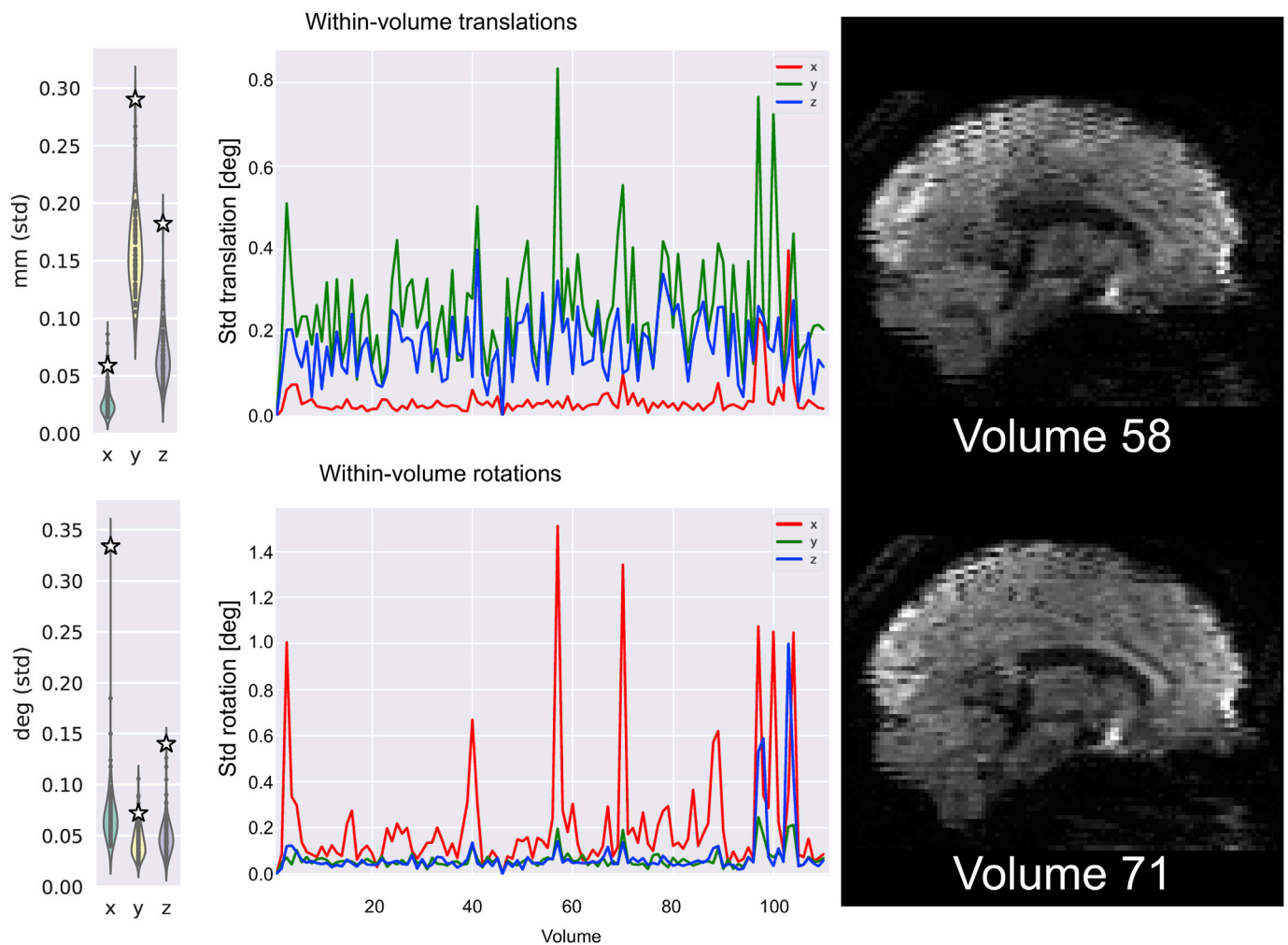
Fig. 4. Single subject with high degree of estimated within-volume motion. This subject's mean standard deviation of the estimated motion parameters (3 translations and 3 rotations) are plotted against their study-wise distributions in the updated single subject report. From the parameters' time-courses shown in the single subject report, two example volumes where the subject has moved the most can easily be extracted and inspected. The two sagittal views prior to correction (not present in the single subject report) show that consecutive slices are misaligned in the distorted, i.e., uncorrected original dataset.
