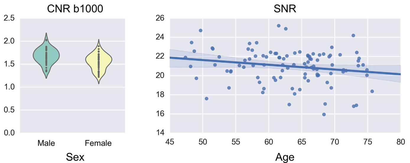
Fig. 8. Differences in quality indices using categorical and continuous variables. Left panel shows differences in the distributions of the average CNR for the b1000 shell between females and males. Right panel shows the average SNR plotted against age. Both panels use the 100 analysed UK Biobank subjects.
