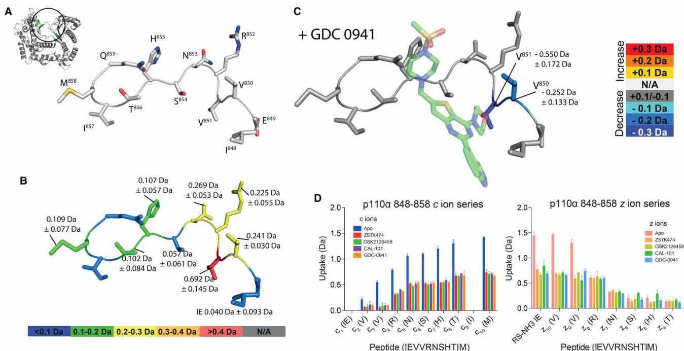
Figure 2. HDX-MS/MS of residues 848–858, detailing compound binding.
