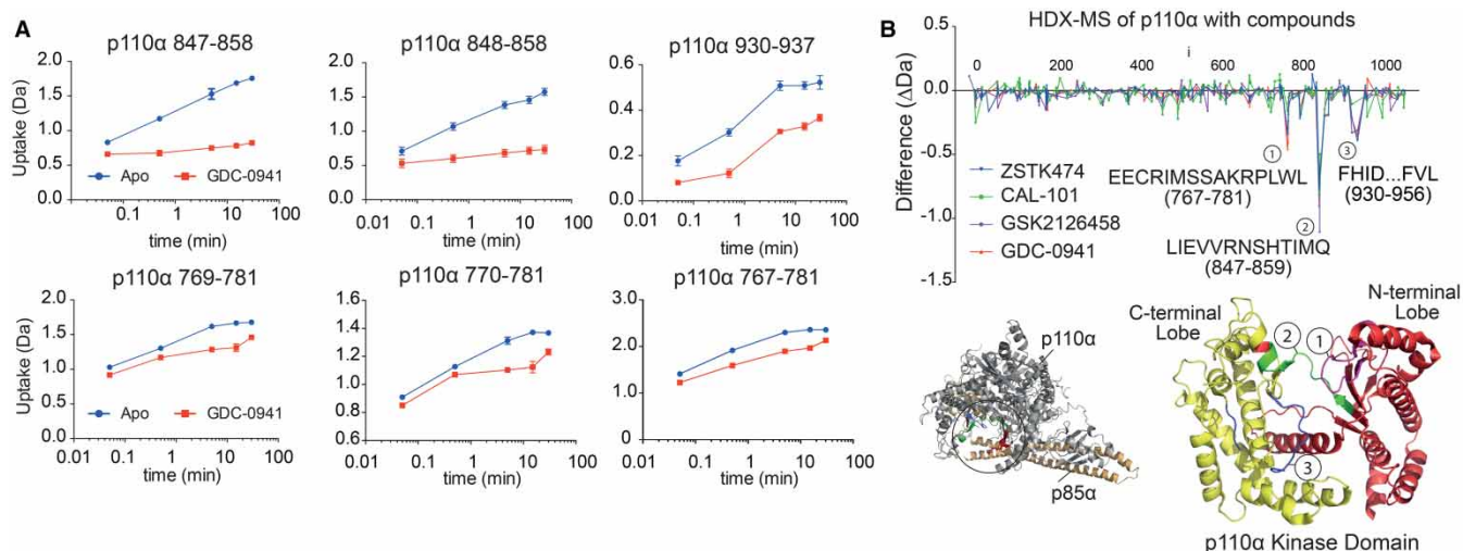
Figure 1. Standard-resolution HDX-MS detailing compound binding.
