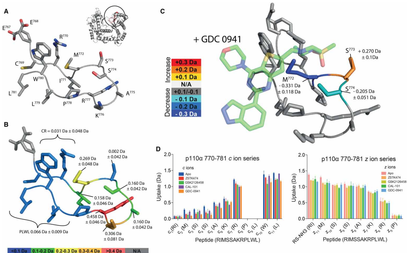
Figure 3. HDX-MS/MS of residues 770–781, detailing compound binding.
