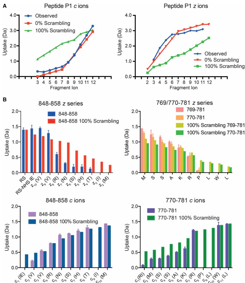
Figure 4. Determination of scrambling.
